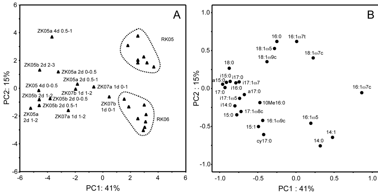
Figure 4. Results of the PCA analysis of the 13 C-labeling patterns in PLFA for all samples with detectable chemoautotrophy showing the site scores (A) and variable scores (B) for the two PCA axes that explained most of the variance. doi:10.1371/journal.pone.0101443.g004
