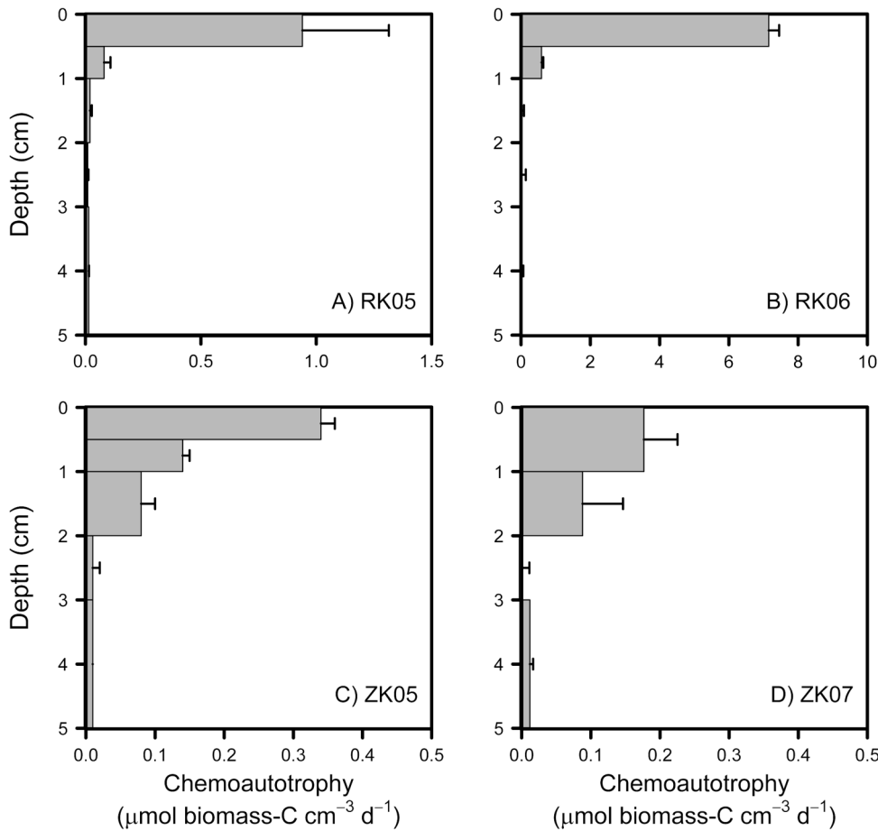
Figure 2. Depth distribution of chemoautotrophy as estimated from ^{13}\text{C} -DIC PLFA labeling in dark incubations for the RK and ZK sediments.
