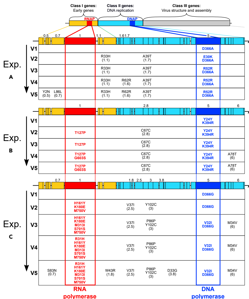
Figure 9. Sequence changes in the viral genome during laboratory evolution
