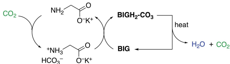
Fig. 10 DAC by CO 2 absorption with aqueous amino acids and carbonate crystallization with BIGs. Reproduced with permission from ref. 45. Copyright (2019) American Chemical Society.
