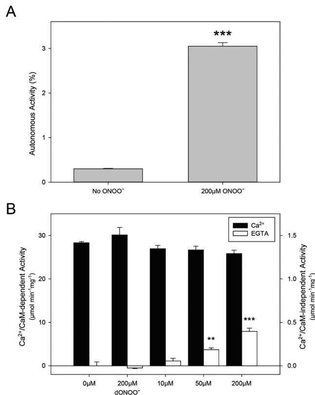
Figure 2. ONOO - induced activation in CaMKII \delta . (A) Percentage of autonomous activity of CaMKII \delta in the presence and absence of 200 \mu M ONOO - . The percentage was calculated from activity of apoenzyme in the presence of EGTA in comparison to maximal activity in the presence of Ca 2+ /CaM. One-way ANOVA using Dunnett's test in comparison to control (No ONOO - ); *** p < 0.001 ( n = 5 ). (B) Kinase activity of CaMKII \delta in the presence of Ca 2+ /CaM (Ca 2+ /CaM-dependent activity) and EGTA (Ca 2+ /CaM independent activity) with increasing concentrations of ONOO - and dONOO - . Activity is represented as specific activity, in \mu mol min -1 mg -1 . Data represent mean values \pm s.e.m from 3 experiments. Note the differences in scale for the two y-axes. One-way ANOVA using Dunnett's post-test compared with control (No ONOO - ); ** p < 0.01 ; *** p < 0.001 .
