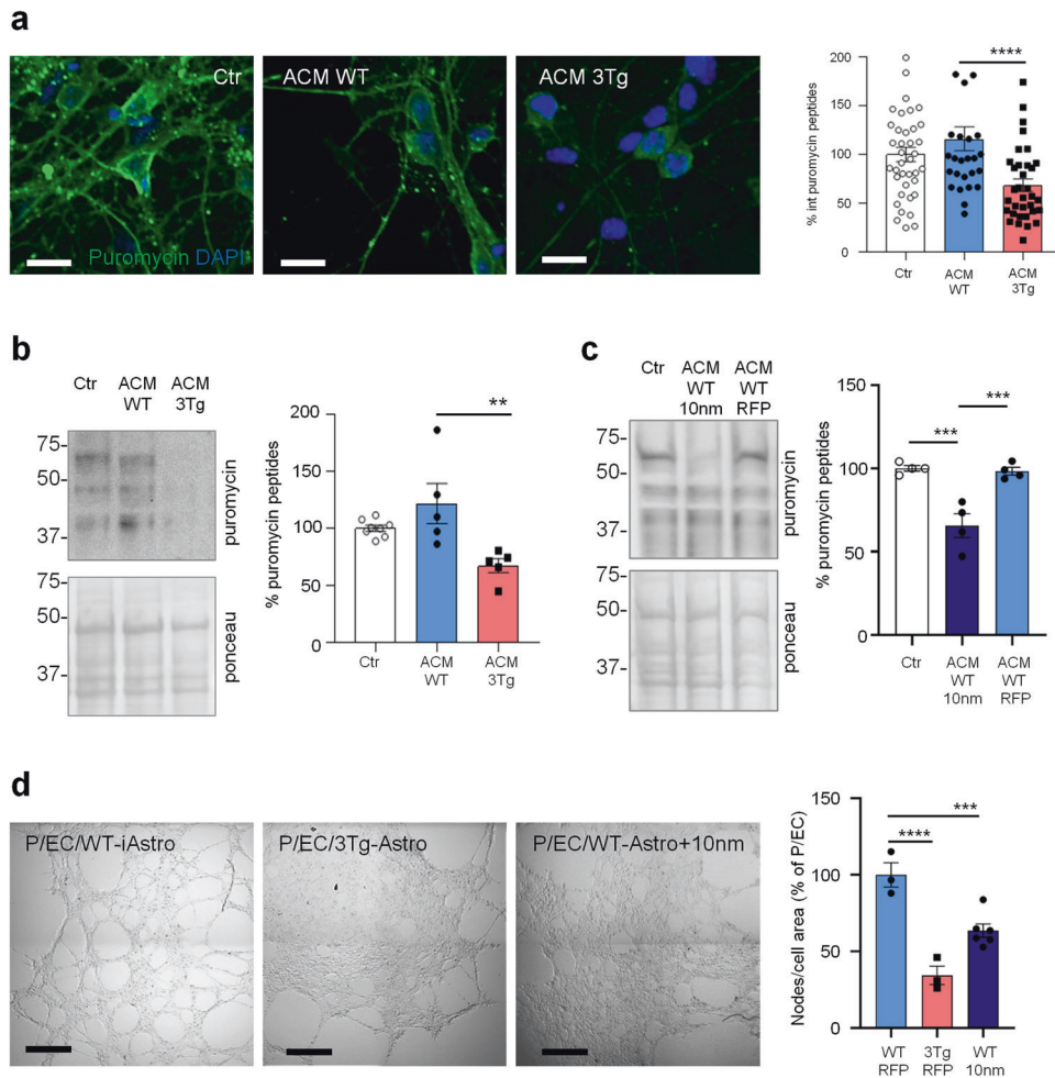
Fig. 7 Compromised homeostatic functions of 3Tg-iAstro. a ACM effects on neuronal protein synthesis. Primary hippocampal neurons were treated with ACM from WT- or 3Tg-iAstro for 6 days (from DIV9 to DIV15) and protein synthesis was evaluated treating cells with 4 \mu M puromycin for 1 h. IF images of anti-puromycin staining (green) and DAPI (blue) were acquired with FV-1000 Olympus laser confocal scanning system, scale bar = 30 \mu m. Data are expressed as mean \pm SEM from n = 39 Ctr, n = 27 ACM WT-iAstro, n = 34 ACM 3Tg-iAstro from four independent cultures; **** p < 0.001 by one-way ANOVA Sidak's multiple comparisons. b WB analysis with anti-puromycin, actin and ponceau staining of neuronal lysates treated as in a . Data are expressed as mean \pm SEM from n = 8 (Ctr) or n = 5 (ACM WT and ACM 3Tg) independent experiments; ** p < 0.01 by one-way ANOVA, Sidak's multiple comparisons. c WB analysis with anti-puromycin and ponceau staining of neuronal lysates treated or not with ACM from WT-iAstro or WT-iAstro expressing 10 nm-EML. Data are expressed as mean \pm SEM of four independent experiments; *** p < 0.001 by one-way ANOVA, Sidak's multiple comparisons. d Co-culture of pericytes and endothelial cells (EC) with either WT-iAstro (P/EC/WT-iAstro) or 3Tg-iAstro (P/EC/3Tg-iAstro) or WT-iAstro expressing the 10 nm-EML (P/EC/WT-iAstro+10nm) cells on a layer of Matrigel. Images were acquired by Zeiss 710 confocal laser scanning microscope, scale bar = 500 \mu m. Data are expressed as mean \pm SEM of n = 3 (WT-RFP and 3Tg-RFP) or n = 6 (WT-10 nm) independent experiments; *** p < 0.001 , **** p < 0.0001 , by one-way ANOVA Sidak's multiple comparisons.
