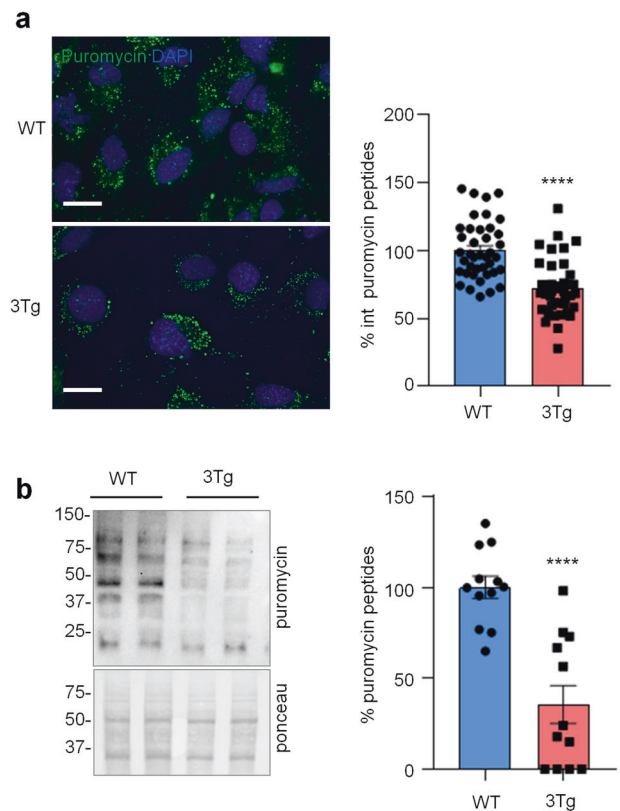
Fig. 1 Protein synthesis analysis in WT- and 3Tg-iAstro cells. a Cells were pulsed with puromycin (4 \mu M, 1.5 h), fixed and analysed by IF with anti-puromycin antibody (green) and with DAPI to stain nuclei (blue). Images were acquired with Leica Thunder imager 3D live cell microscope, scale bar = 25 \mu m. Data are expressed as mean \pm SEM, WT-iAstro cells n = 40 , 3Tg-iAstro cells n = 40 , from 4 independent experiments; **** p < 0.05 by unpaired t -test. b WB with anti-puromycin antibody and ponceau staining on cells treated with 4 \mu M puromycin. Data are expressed as mean \pm SEM of 12 independent experiments; **** p < 0.0001 by unpaired t -test.
