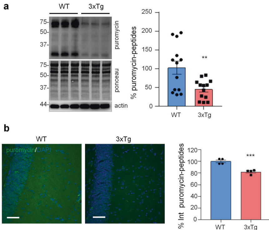
Fig. 5 Protein synthesis analysis in WT and 3xTg-AD mice. WT and 3xTg-AD mice were i.p. injected with 225 mg/Kg of puromycin and sacrificed 1.5 h post-injection. a WB with anti-puromycin, anti-actin antibodies, and ponceau staining on hippocampal homogenates. Data are expressed as mean \pm SEM of 13 independent WB from two mice per genotype. ** p < 0.01 , unpaired t -test. b IF with anti-puromycin antibody (green) and DAPI (blue) of hippocampal brain slices. Data are expressed as mean \pm SEM of four sections collected from two mice per genotype. Scale bar = 50 \mu m.
