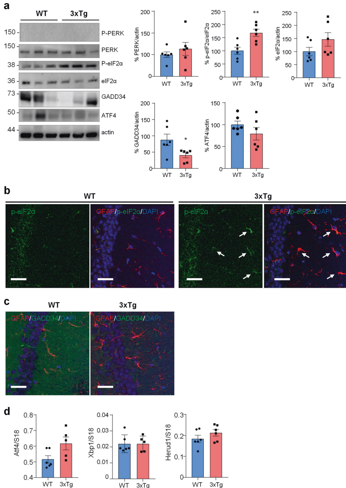
Fig. 6 ER stress/UPR pathway in WT and 3xTg-AD mice. a WB analysis with anti-PERK, p-eIF2 \alpha , eIF2 \alpha , GADD34, ATF4 and actin on hippocampal homogenates of WT and 3xTg-AD (3xTg) mice. Data are expressed as mean \pm SEM of six independent experiments; * p < 0.05; ** p < 0.01 by unpaired t -test. b, c Co-localization of p-eIF2 \alpha and GADD34 with GFAP and analysis on WT and 3xTg hippocampi. b IF on 40 \mu m thick brain slices with anti-GFAP (red), p-eIF2 \alpha (green) and DAPI (blue). Arrows indicate p-eIF2 \alpha -expressing GFAP-positive astrocytes. c IF on 40 \mu m brain slices with anti-GFAP (red) and GADD34 (green) and DAPI (blue). Images were acquire using Leica SP8 LIGHTNING Confocal Microscope imaging systems, scale bar = 25 \mu m. d qPCR of Atf4, Xbp1s and Herpud1 on the hippocampi of WT and 3xTg mice. Data are expressed as mean \pm SEM of 5–6 independent experiments, unpaired t -test analysis.
