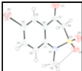
Fig. 1. The title compound, with the atom-numbering scheme. The displacement ellipsoids are drawn at the 50% probability level. The H-atoms are shown by small circles of arbitrary radius. The dotted lines show the intramolecular H-bonds.
