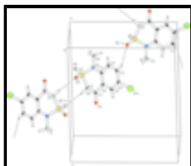
Fig. 2. A section of the title structure showing the dimers bind by the hydrogen bonds.
