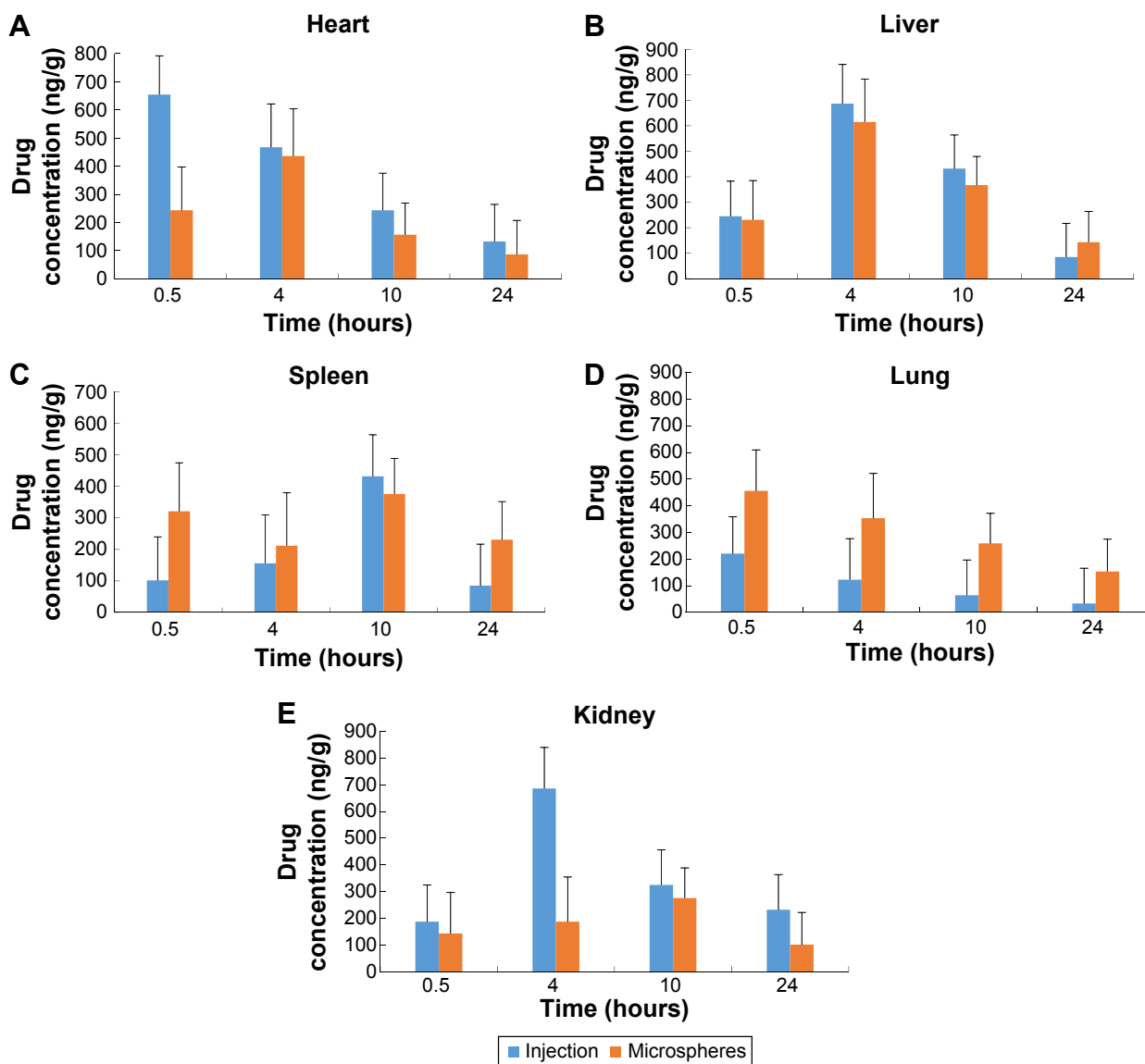
Figure 4 Concentrations of TED in mice tissues after intravenous administration of TED-loaded chitosan microspheres and TED injection (n=6). Note: Results for (A) heart, (B) liver, (C) spleen, (D) lung, (E) and kidney tissues. Abbreviation: TED, tetrandrine.
