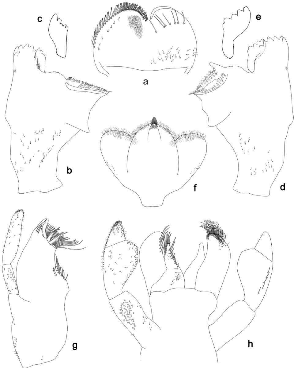
Figure 24. Labiobaetis magnovaldus sp. n., larva morphology: a Labrum b Right mandible c Right prosthema d Left mandible e Left prosthema f Hypopharynx g Maxilla h Labium.
