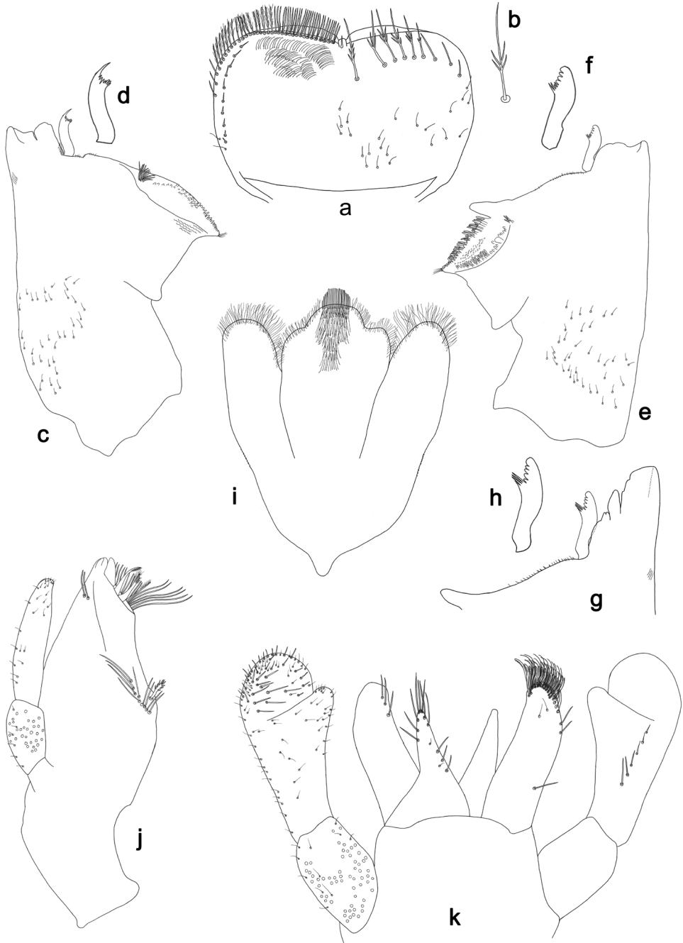
Figure 48. Labiobaetis dendrisetis sp. n., larva morphology: a Labrum b Labrum dorsal, submarginal seta c Right mandible, denticles outworn d Right prosthema e Left mandible, denticles outworn f Left prosthema g Left mandible, denticles unused h Left prosthema i Hypopharynx j Maxilla k Labium.
