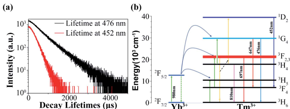
Fig. 8 (a) Decay curves for ^1\text{D}_2 \rightarrow ^3\text{F}_4 (452 nm) and ^1\text{G}_4 \rightarrow ^3\text{H}_6 (476 nm) emission of UCNPMF excited at 980 nm. (b) Energy diagram of \text{Yb}^{3+} and \text{Tm}^{3+} with the possible upconversion mechanism under 980 nm excitation.
