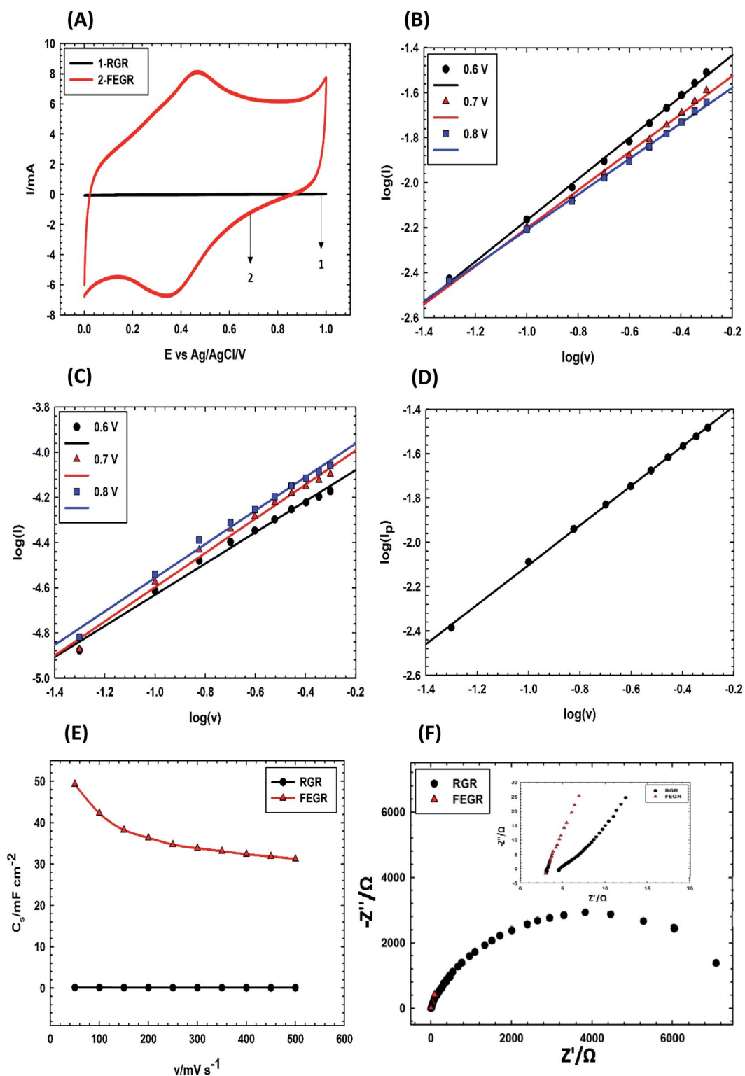
Fig. 4 (A) CVs of RGR (black line), and FEGR (red line) electrodes at a potential scan rate of 100 mV s -1 . The variation of (log I ) with (log v ) at different potentials (0.6, 0.7, and 0.8 V) for (B) RGR electrode, and (C) FEGR electrode. (D) The variation of (log I pa ) with (log v ) of FEGR electrode. (E) The variation C s with v of RGR (black line) and FEGR (red line) electrodes. (F) Nyquist plots of RGR (black line) and FEGR (red line) electrodes at OCP and its inset at high-frequency region.
