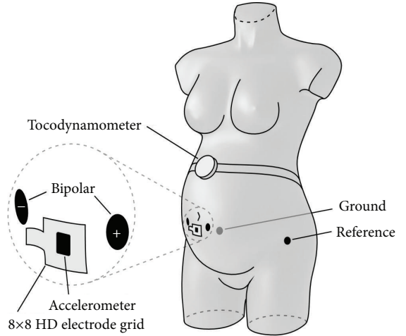
FIGURE 1: Measurement setup showing the position of all abdominal sensors.
