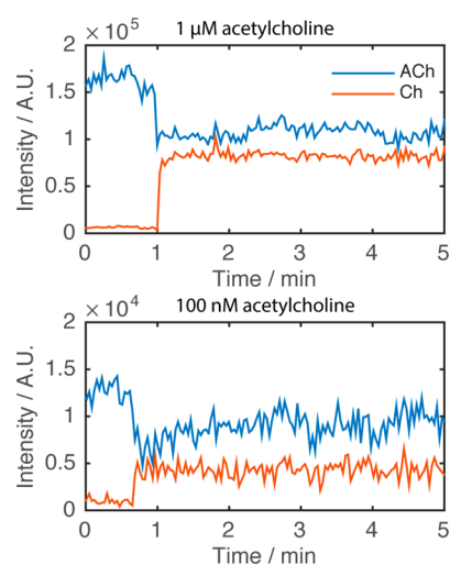
Figure 4. Representative traces of real-time mass spectrometry monitoring conversion of acetylcholine (ACh, m/z 146.1176) into choline (Ch, m/z 104.1070) by acetylcholinesterase. Use of a large capillary inner diameter (o.d. 350 \mu\text{m} , i.d. 200 \mu\text{m} ) and higher flow rate ( q_{\text{in}} = 8 \mu\text{L}/\text{min} , q_{\text{out}} = 10 \mu\text{L}/\text{min} ) leads to a low surface-to-volume ratio in combination with less time for substrate diffusion, resulting in lower conversion compared to what is obtained with smaller capillaries and lower flow rates.
