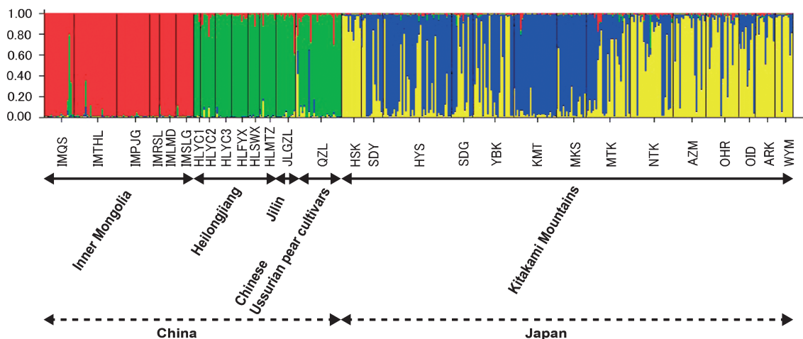
Fig. 3. Percentage membership of genotypes to clusters (q value) inferred at K = 4 (independent model) applying all samples without local varieties originated from P. ussuriensis var. aromaticata to STRUCTURE analysis. Each genotype is represented by a vertical line divided into colored segments. The length of the vertical lines indicates the proportion of genome attributed to the inferred clusters.
