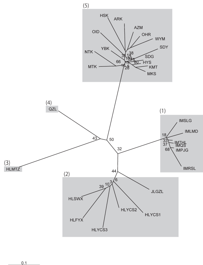
Fig. 4. Unrooted neighbor-joining tree based on Nei's DA distance value among populations. The number of points of divergence represents bootstrap values. The six populations (IMQS, IMTHL, IMPJG, IMRSL, IMLMD, and IMSLG) originating from Inner Mongolia. (2) The 5 populations (HLYCS3, HLFYX, HLSWX, HLYCS2, and HLYCS1) from Heilongjiang. (3) HLMTZ from Mudanjiang, Heilongjiang. (4) The cultivated Ussurian pears (QZL) were combined. (5) The 14 populations (HSK, SDY, HYS, SDG, YBK, KMT, MKS, MTK, NTK, AZM, OHR, OID, ARK, and WYM) originating from Kitakami Mountains in Japan.
