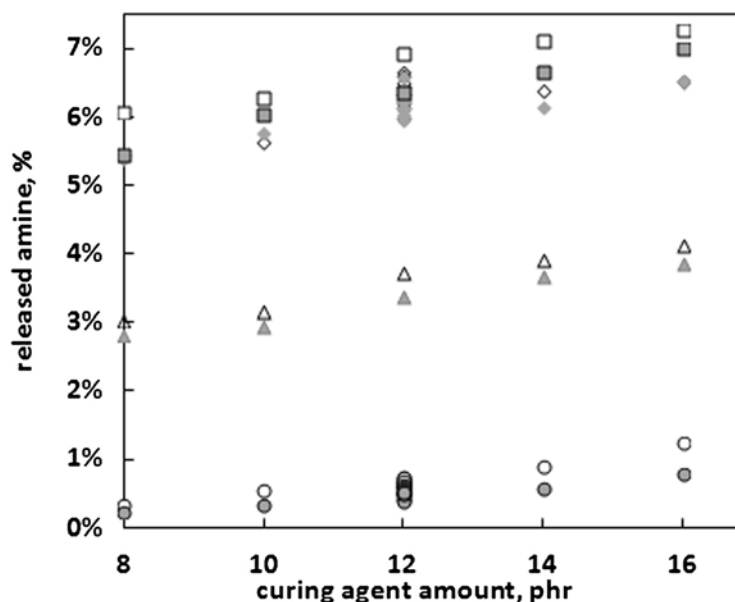
Figure 2 Amounts of residual amine extracted from cured epoxy resin with water (◇), 95% ethanol (○), 10% ethanol (△) and 3% acetic acid (□). The determinations performed using calibration with 527 nm absorbance for pellets after 24 hours of curing (white) and pellets after six months in room temperature (grey).
