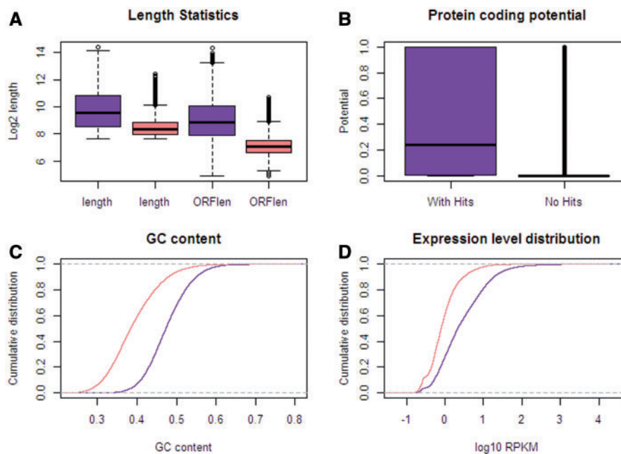
Fig. 1. —Comparison between the set of unigenes with and without BLAST-hits. (A) Overall length and longest ORF length statistics, (B) protein-coding potential determined by CPAT, (C) distribution of GC content, and (D) distribution of normalized expression level. Purple color, with BLAST hit; pink, without BLAST hit.
