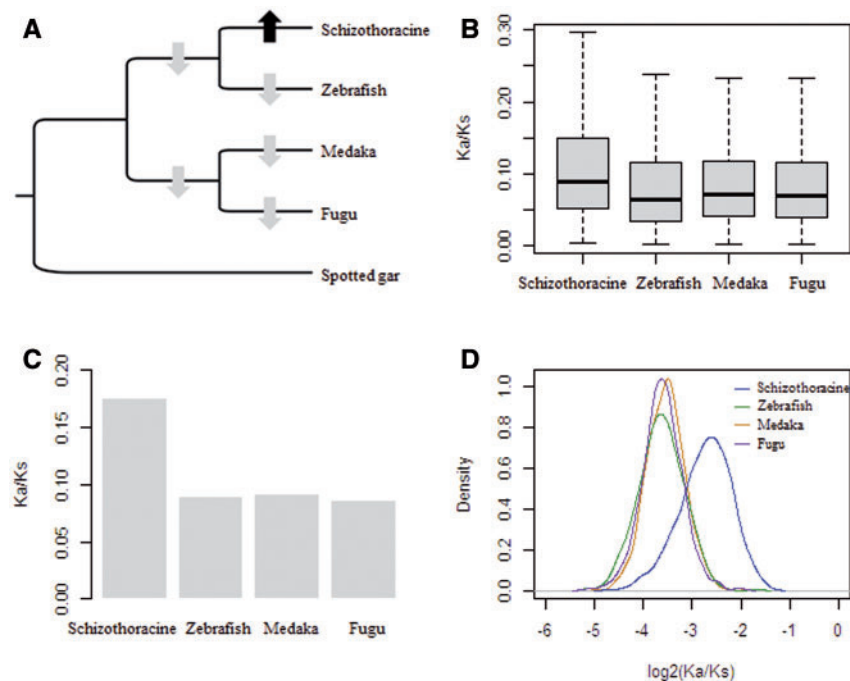
FIG. 2. —Phylogenetic tree used in this study (A) and branch specific Ka/Ks ratios obtained from different data sets (B–D). Gray and black arrows in (A) indicate decreased or increased terminal Ka/Ks ratios compared with the ancestral branch. The Ka/Ks ratios for terminal branches were estimated from each ortholog (B), concatenated all orthologs (C), and 1,000 concatenated alignments constructed from ten randomly chosen orthologs (D).
