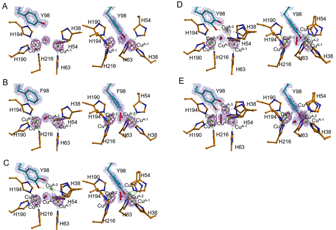
Fig 3. Electron density around the dicopper center and 98th residue in the caddie protein obtained by the NH 2 OH treatment to the met 2 -form crystals. (A) was obtained by the anaerobic soaking of the wild-type complex with CuSO 4 and NH 2 OH for 2 h (ST1). (B) was obtained by the aerobic soaking of the Y98F-mutated complex for 2 h (ST2). (C), (D), and (E) were obtained by the aerobic soaking of the wild-type complex for 10 min (ST3), 20 min (ST4), and 2 h (ST5), respectively. The 2F o -F c electron density map around Tyr 98 (or Phe 98 ) in the caddie protein, Cu A , Cu B , and bridging molecules was contoured at 1.5 σ (blue), 2.5 σ (purple), 3.5 σ (orchid), 4.5 σ (violet red), and 5.5 σ (red). The right panels are different views of the left panels. Electron densities for a hydroxyl group newly added to the Tyr 98 residue in ST3 or ST4 are invisible in the present maps because of the low occupancy. H, histidine; F, phenylalanine; Y, tyrosine; Y98F-mutated complex, complex between tyrosinase and the mutated caddie, in which the Tyr 98 residue is replaced with phenylalanine.
