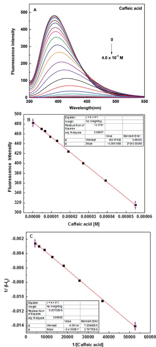
Fig. 5 (A) Fluorescence spectra of sensor 5c ( 1 \times 10^{-5} M) in the presence of different concentrations of caffeic acid in PBS (pH 7.4) solution, at room temperature; (B) the photograph of sensor 5c linear range; (C) Benesi–Hildebrand plot of sensor 5c 1/(I - I_0) versus 1/[\text{Caffeic acid}] .
