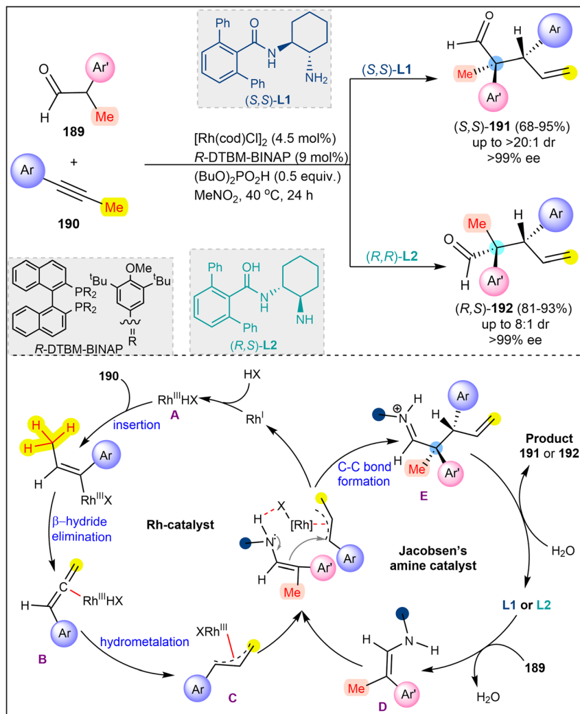
Scheme 46 Chiral Jacobsen's amine-dependent stereodivergent synthesis of α-β-chiral homoallylic ketones and through Rh-hydride catalyzed coupling of α-branched aldehydes with alkynes.
