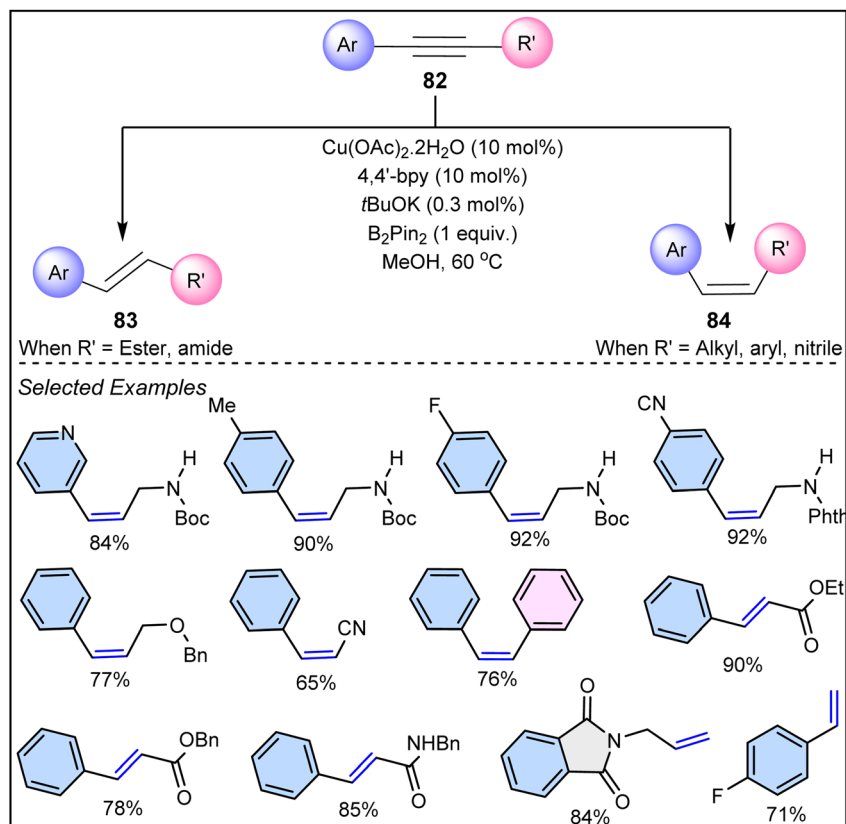
Scheme 20 \text{Cu(OAc)}_2 and nitrogen-based ligand catalyzed semi-hydrogenation of alkynes.
