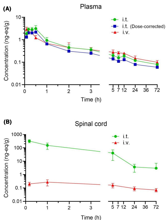
FIGURE 7 Drug-related total and dose-corrected (after intrathecal [i.t.] administration in plasma) radioactivity in rat plasma (A) and spinal cord (B) converted to mass equivalents of 3 H-Fadolmidine base after an intrathecal or intravenous (i.v.) dose of about 3 µg/kg of the compound (hydrochloride). For the dose-correction, the radioactive doses were 4.198 and 2.918 MBq/kg after intrathecal and intravenous administration, respectively. Values are presented as Mean ± SD. ( n = 6 per time point)
