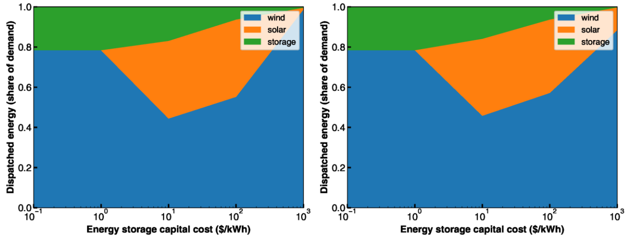
Figure S23. Effect of storage cost on relative shares of dispatched electricity (that directly meets the electricity demand) in the least-cost VRE/storage systems for the year 2015. Curtailed generation of wind and solar electricity are excluded in this figure but available in Figure S24. The baseline technology scenario (Table S2) is assumed. The left panel shows the optimization results for 100% resource adequacy, and the right panel shows those for at least 99.97% resource adequacy. The total share of dispatched energy from wind, solar, and energy storage is 99.97% in the right panel. Related to Figure 2.
