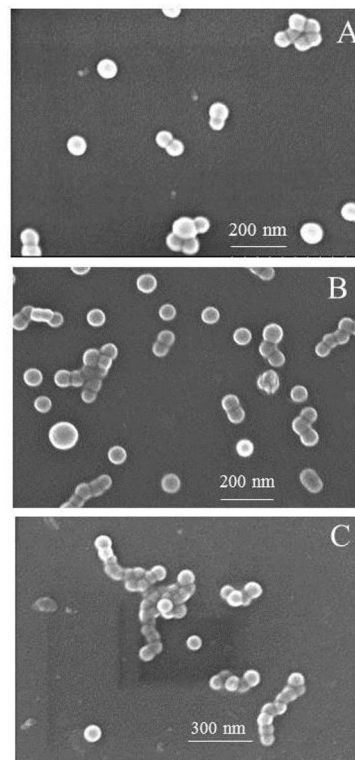
Fig. 7 SEM microscopy of the self-assembled micelles of iPS-b-1,4-trans-PBD (Entry 6 in Table 1) in n -dodecane after prepared for, (A) 0 day, (B) 7 day, (C) 14 day.
