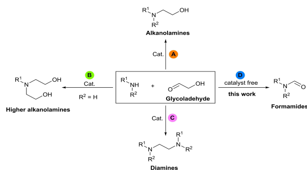
Scheme 1. Reactions of secondary amines with glycolaldehyde.
