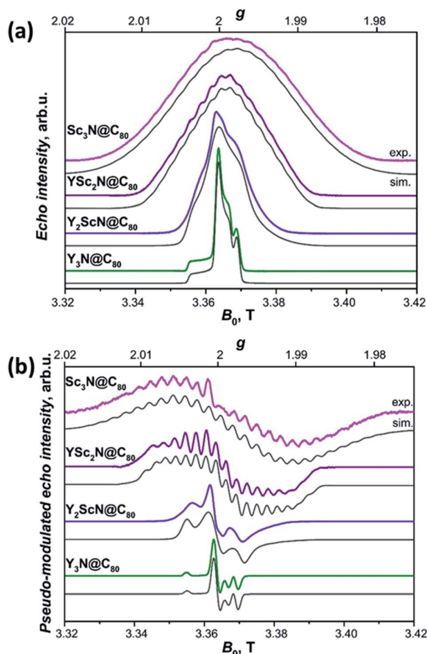
Fig. 10 (a) W-band ESE-detected EPR spectra of the Y_3N@C_{80} (green line), Y_2ScN@C_{80} (violet line), YSc_2N@C_{80} (purple line) and Sc_3N@C_{80} (magenta line) excited triplet states recorded in frozen toluene- d_8 solution at 20 K under continuous 510 nm laser illumination. Grey lines represent EPR spectra calculated using the spin Hamiltonian in eqn (2) and the magnetic parameters summarized in Table 2. (b) The same ESE EPR spectra processed by a field pseudo-modulation procedure (modulation amplitude of 1.5 mT) to resemble continuous-wave (CW) EPR spectra. The ^{45}Sc hyperfine multiplets are clearly resolved in the YSc_2N@C_{80} and Sc_3N@C_{80} traces. Reduced spin density on Y atoms together with smaller nuclear g -factor ( g_n = -0.27 for ^{89}Y versus g_n = 1.36 for ^{45}Sc ) lead to much smaller ^{89}Y hyperfine couplings, which cannot be resolved in the EPR spectra.
