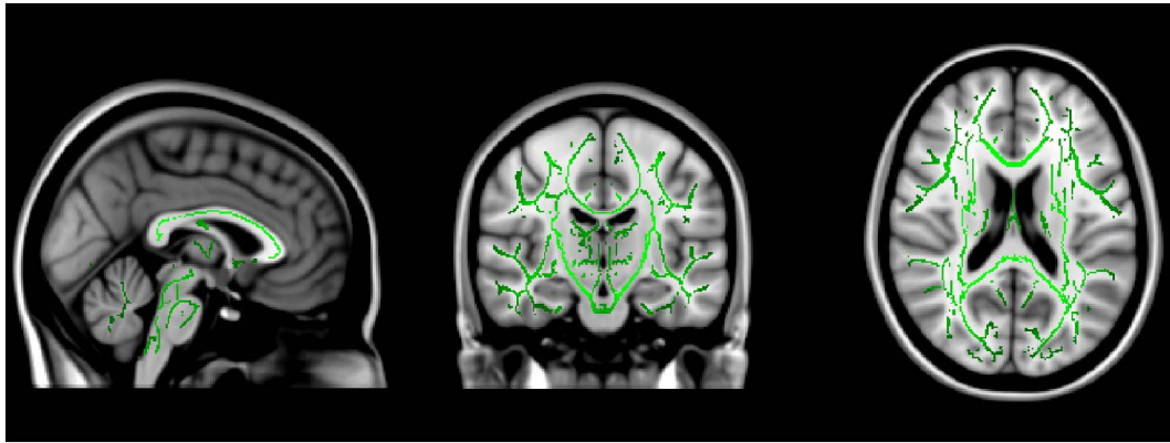
Fig. 1. White matter structures showing no regions with significantly higher FA in controls compared to the clinical groups ( p < 0.05 , corrected for multiple comparisons). Green voxels show the mean FA white matter skeleton for these participants. Template image is the standard MNI152 brain.
