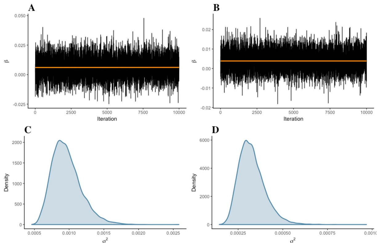
Fig. 7. Trace plot and marginal density for parameter \beta of the difference between groups (Dyslexics vs. Non-dyslexics) in mean FA values. (A–C) Left AF. (B–D) Right AF. Estimates were generated from 10,000 iterations, in one chain, with thinning interval of one (i.e., no data point discarded). Both trace plots (the values parameter \beta took during the runtime of the chain) and marginal densities (smoothed histograms of parameter \beta values) indicated that the difference between groups was practically null.
