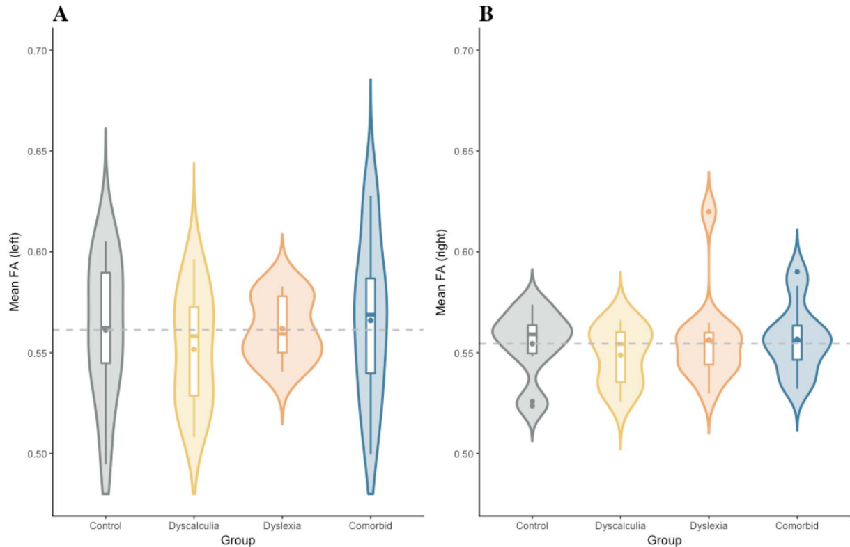
Fig. 5. Descriptive plots of FA values across the arcuate fasciculus for all four groups (Control, Dyscalculia, Dyslexia, Comorbid). For each group, the plot shows the distribution of gain scores (violin) together with the mean (box central dot), median (box central line), first and third quartile (box edges), minimum and maximum (whiskers), and outliers (outside dots). The dashed line references the mean value for the control group. (A) Left hemisphere. (B) Right hemisphere.
