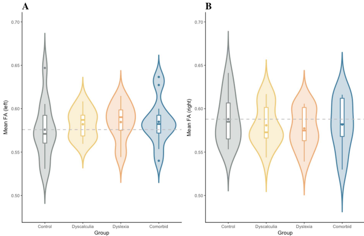
Fig. 2. Descriptive plots of FA values across the corona radiata for all four groups (Control, Dyscalculia, Dyslexia, Comorbid). For each group, the plot shows the distribution of gain scores (violin) together with the mean (box central dot), median (box central line), first and third quartile (box edges), minimum and maximum (whiskers), and outliers (outside dots). The dashed line references the mean value for the control group. (A) Left hemisphere. (B) Right hemisphere.
