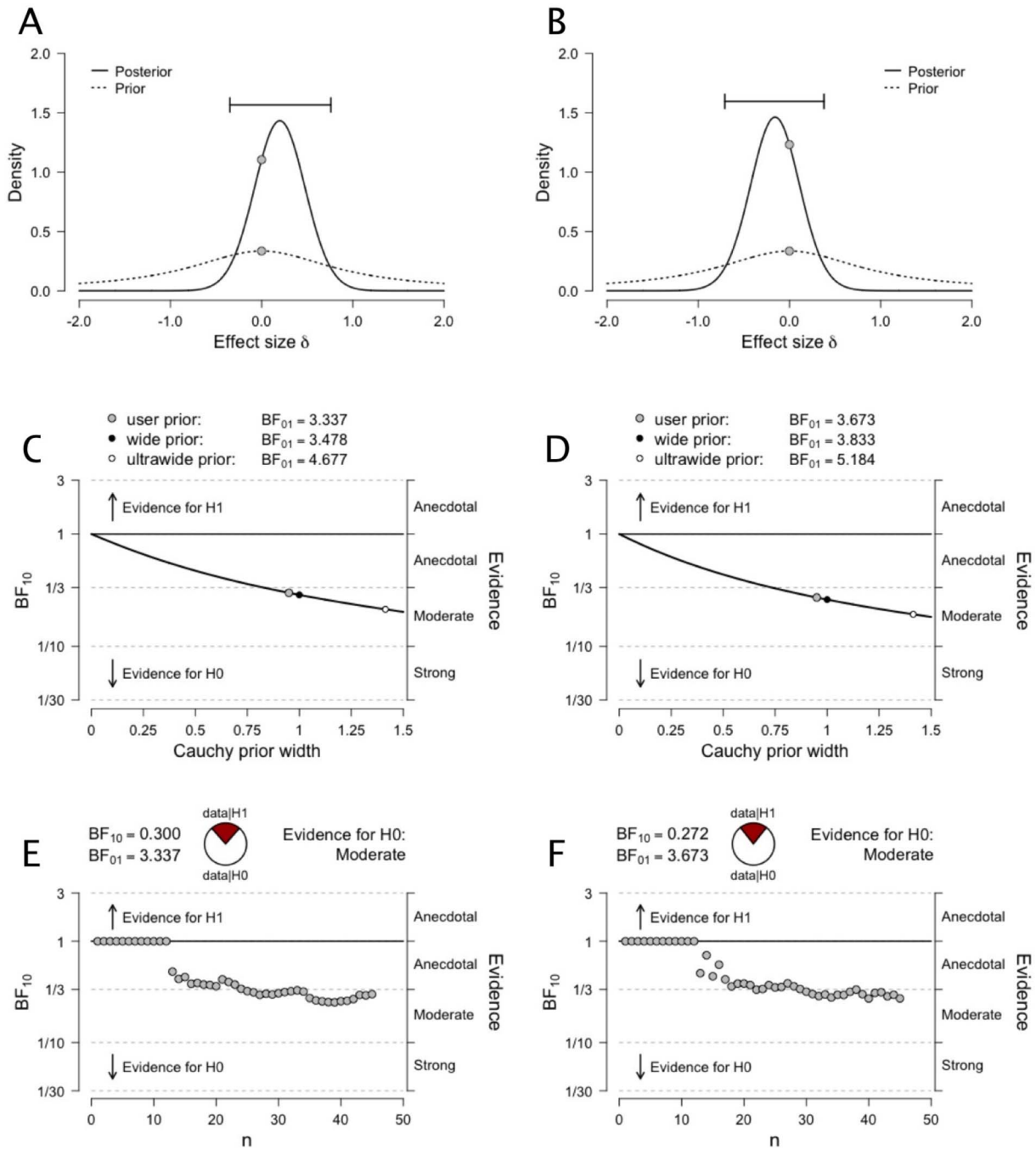
Fig. 3. (A–B) Prior and posterior distributions for the comparison between Groups (Dyslexics vs. Non-dyslexics) for the left and right CR mean FA values. (C–D) Bayes factor robustness analyses for the comparison between Groups (Dyslexics vs. Non-dyslexics) for the left and right CR mean FA values. The figure shows our default prior (gray dot), as well as wide and ultrawide priors (black and white dots, respectively). (E–F) Sequential analysis showing the strength of evidence (as expressed by BF_{10} ) as N increases, for the left and right CR mean FA values. Note that data points are ordered by group.
