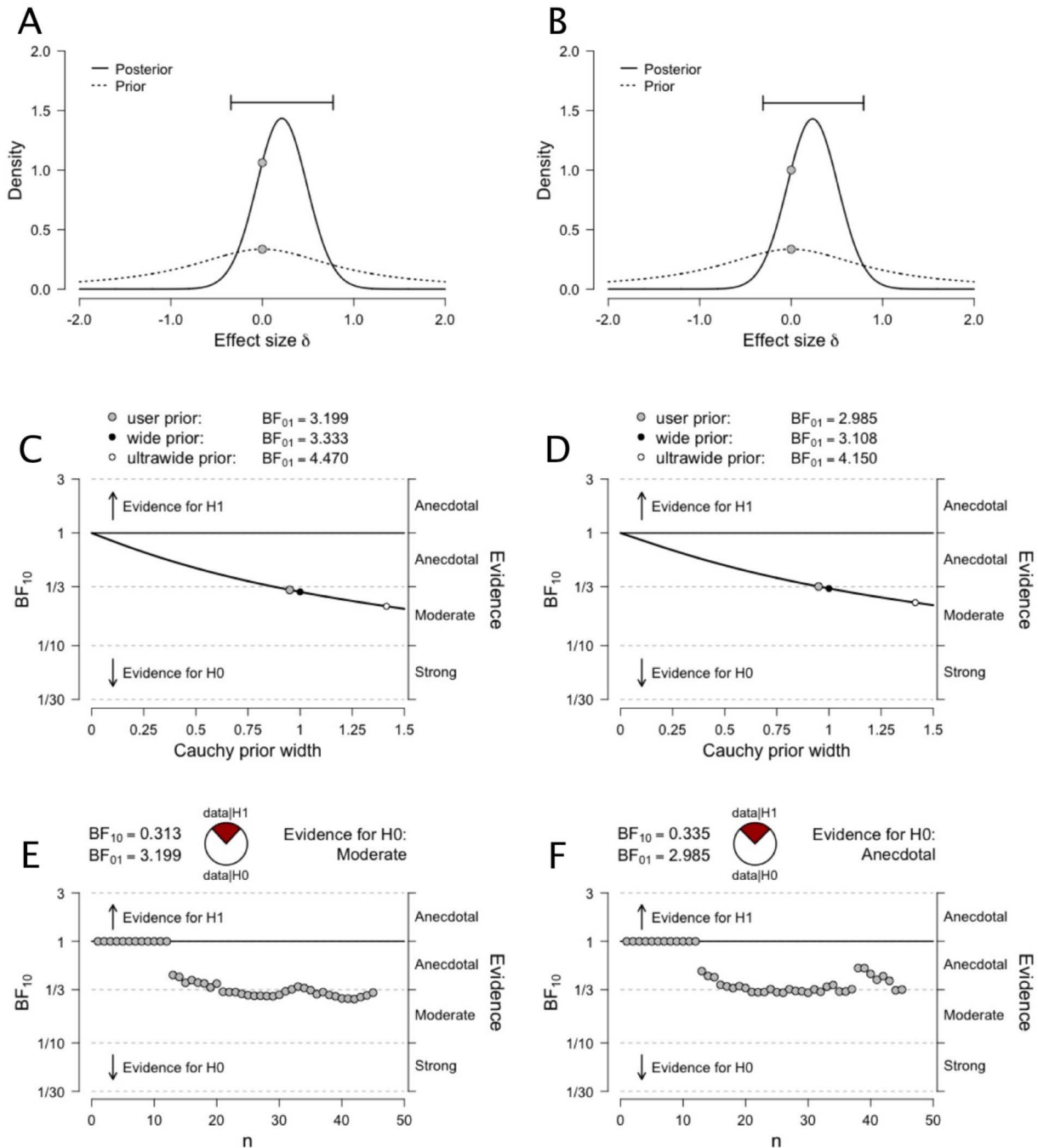
Fig. 6. (A–B) Prior and posterior distributions for the comparison between Groups (Dyslexics vs. Non-dyslexics) for the left and right AF mean FA values. (C–D) Bayes factor robustness analyses for the comparison between Groups (Dyslexics vs. Non-dyslexics) for the left and right AF mean FA values. The figure shows our default prior (gray dot), as well as wide and ultrawide priors (black and white dots, respectively). (E–F) Sequential analysis showing the strength of evidence (as expressed by BF_{10} ) as N increases, for the left and right AF mean FA values. Note that data points are ordered by group.
