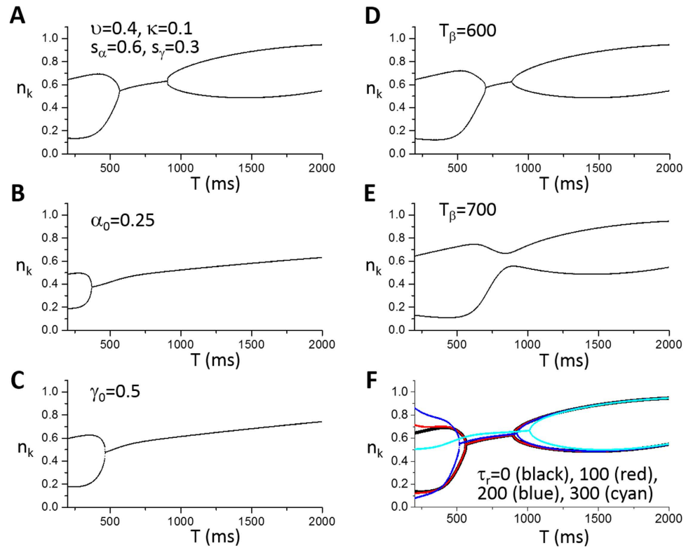
Figure 6. Effects of spark properties on dynamics. Shown in each panel is the number of sparks ( n_k ) versus pacing period ( T ) from the iterated map model (Eqs 7 and 8). (A) Control, which was modified from Fig. 5A by changing v and \kappa ( v=0.4 and \kappa=0.1 ). (B) Reduced primary spark probability ( \alpha_0=0.25 ). (C). Reduced recruitment ( \gamma_0=0.5 ). (D) T_\beta=600 ms. (E) T_\beta=700 ms. (F) In the presence of spark amplitude restitution for \tau_r=0 ms (black, the same as A), 100 ms (red), 200 ms (blue), and 300 ms (cyan).
