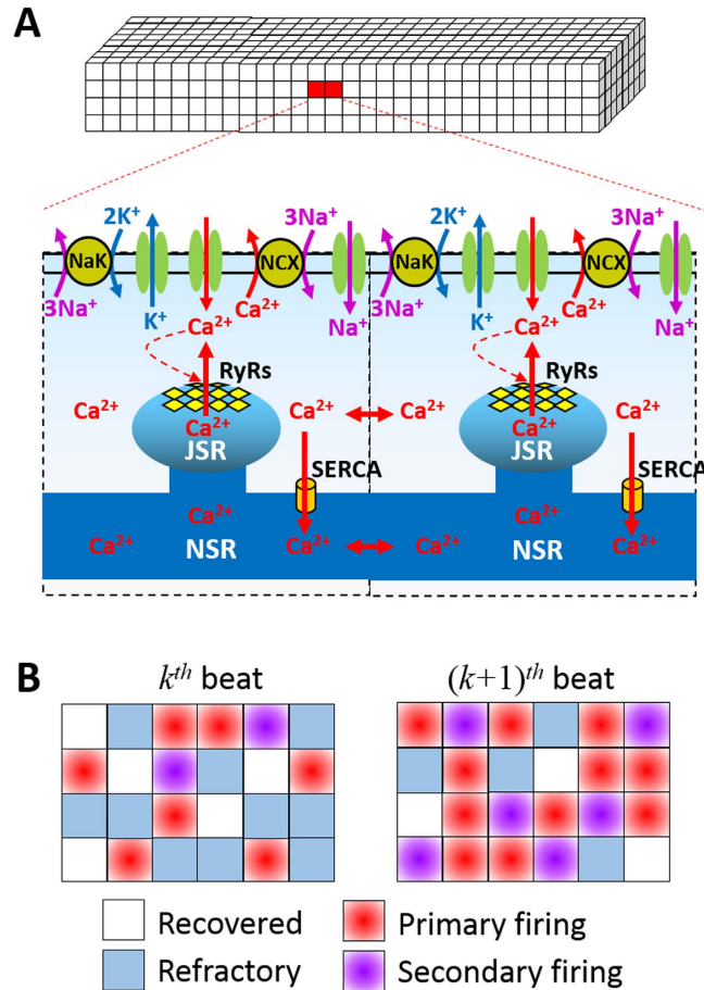
Figure 2. Schematic diagrams for spatiotemporal Ca 2+ cycling in ventricular myocytes. (A) Schematic diagrams of CRU network representing a ventricular myocyte, excitation-contraction coupling in a CRU, and CRU coupling via Ca 2+ diffusion. JSR—junctional SR and NSR—network SR. (B) Schematic CRU firing patterns.
