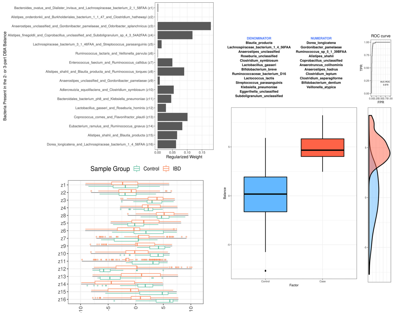
FIG 4 The most important distal DBA balances (left) compared with the results from selbal (right). In the top left portion are the regularized weights for each distal balance. In the bottom left portion is the distribution of samples for each balance irrespective of weight. The distal DBA classifier uses the weighted sum of these balances to make its prediction. In the right portion is the distribution of a single balance as selected by selbal. Many of the same variables are represented in both sets. DBA selects multiple simple balances instead of one complex balance. All panels generated using the 2a data set, comparing inflammatory bowel disease (in red) with healthy controls (in blue).
