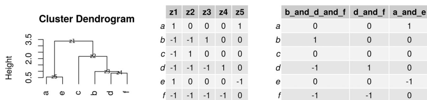
FIG 2 How a balance dendrogram relates to a serial binary partition (SBP) matrix. The left portion shows a dendrogram clustering the similarity between 6 components, where the first branch in the dendrogram refers to the first balance (i.e., a and e versus c, b, d, and f). The middle portion shows the corresponding SBP with 5 balances (columns) and the components involved in each log contrast (rows). The right portion shows the distal 2- and 3-part balances.
