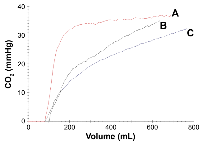
Figure 1 Illustrative curves constructed with mean values of each group. Notes: (A) Control group (ETCO 2 =36 mmHg; Slp3=7.3 mmHg/L; V e =693.2±245.9 mL); (B) airways diseases group (ETCO 2 =39.0±6.7 mmHg; Slp3=37.1±15.5 mmHg/L; V e =508.5 mL); (C) emphysema group (ETCO 2 =33.7±6.8 mmHg; Slp3=28.6±12.7 mmHg/L; V e =652.1 mL). Data from Veronez et al. 15 Abbreviations: ETCO 2 , end-tidal CO 2 ; Slp3, slope of phase 3; V e , expired volume.
