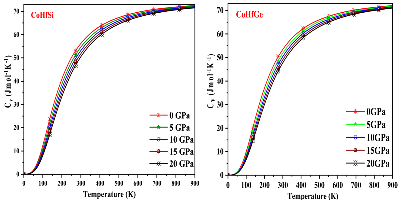
Fig. 14 The variation of specific heat with the temperature at different pressure of CoHfSi and CoHfGe half Heuster alloys.
