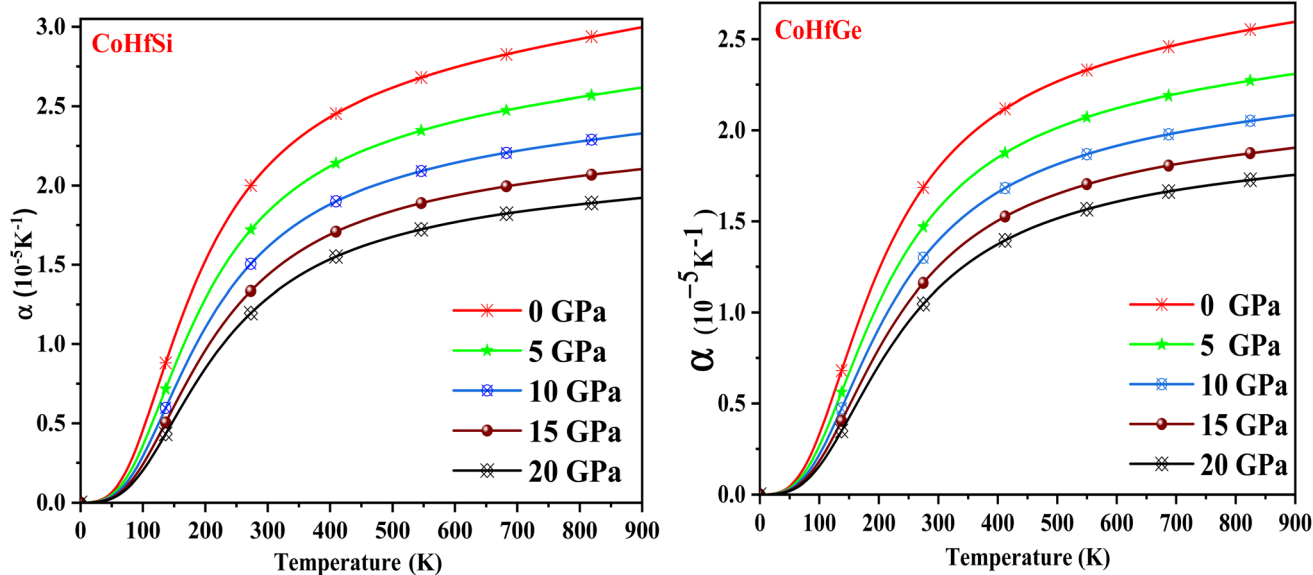
Fig. 15 The variation of thermal expansion coefficient with the temperature at different pressure of CoHfSi and CoHfGe half Heusler alloys.
