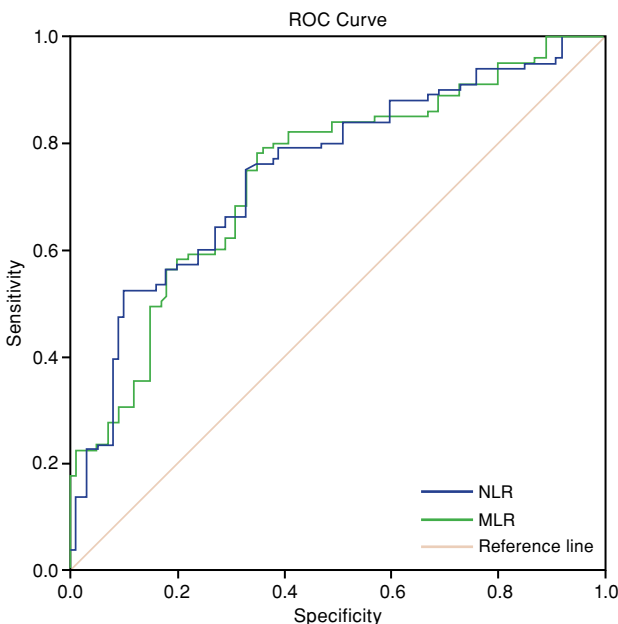
FIGURE 1. Receiver operating characteristic curves for NLR and MLR. NLR: Neutrophil-to-lymphocyte ratio; MLR: Monocyte-to-lymphocyte ratio; ROC: Receiver operating characteristic.
