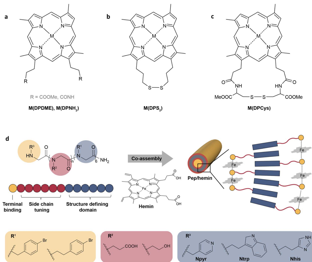
Fig. 3 (a–c) The structures of metallo-deuteroporphyrins designed for the catalytic depolymerization of lignin. 91 Adapted with permission from ref. 91. Copyright 2015 Wiley-VCH. (d) The schematic representation of self-assembled peptoid/hemin nanotubes. 92 Adapted with permission from ref. 92. Copyright 2022 Springer Nature.
