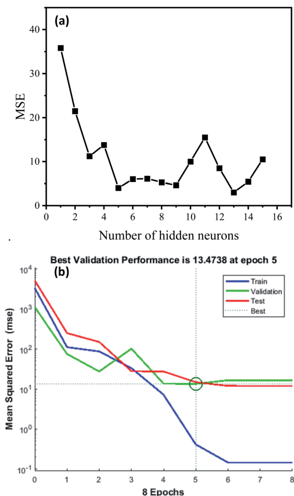
Fig. 9 (a) MSE plot for different numbers of neurons in the hidden layer (1–15) for the response of SDBS removal efficiency; (b) ANN performance validation plot.
