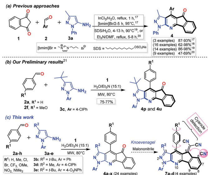
Scheme 1 Synthesis of indeno[1,2- b ]pyrazolo[4,3- e ]pyridin-5-ones 4 and 4a-x.
