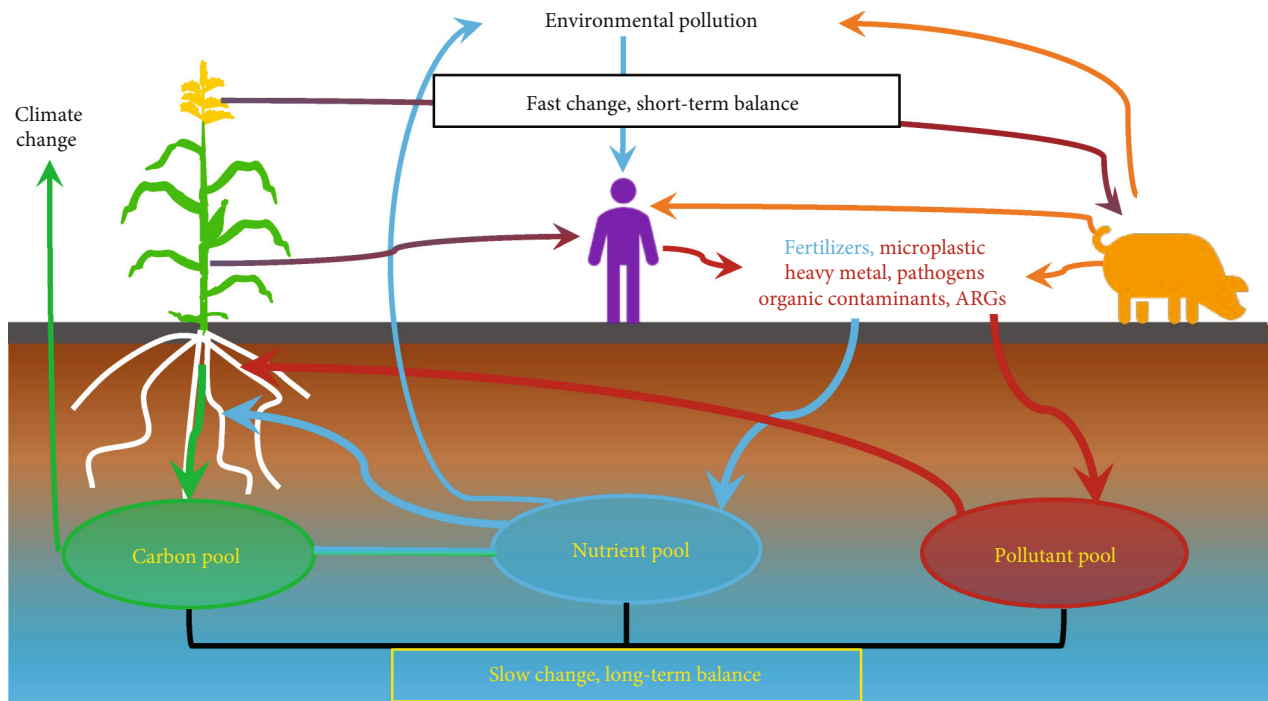
FIGURE 1: Diagram of soil-food-environment-human nexus. The mismatch of fast changes derived from human activities and slow changes derived from soil processes require the protection of soils urgently. Soil pollution can cascade through the food chain and environment to humans and damage human health ultimately. ARGs refer to antibiotic resistance genes.
