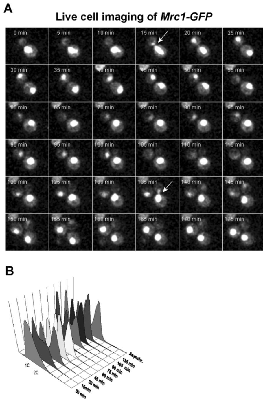
Figure 3 Nuclear presence of Mrc1 throughout the cell cycle. (A) Time-lapse live cell imaging of MRC1-GFP yeast cell throughout the cell cycle. The arrows indicate the characteristic anaphase nuclear morphology of the cell. The frames situated between two arrows encompass of one entire cell cycle. (B) FACS analysis of MRC1-GFP yeast cells after release from 100 mM HU arrest.
