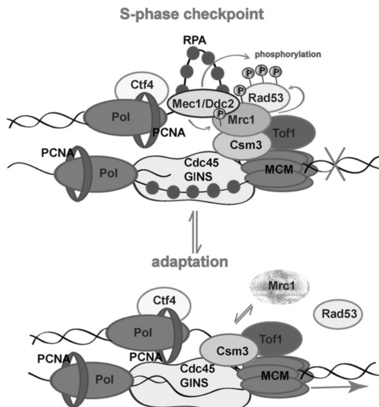
Figure 6 The role of Mrc1 for the duration of the S-phase checkpoint arrest.
