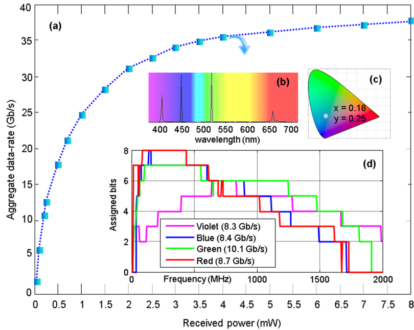
Figure 3. WDM results for maximum data-rate. (a) Received optical power in total vs. measured aggregate data-rate using channel adaptive OFDM, where the power proportion is adjusted to maximise the data-rate for a given power level. (b) Optical spectrum, (c) CIE colour coordinate, and (d) Assigned bits for each colour leading to 35.6 Gb/s (BER <math>3.8 \times 10^{-3}</math>).
