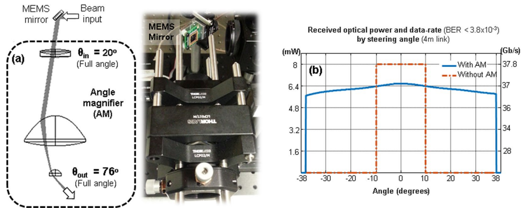
Figure 4. Coverage. (a) Angle magnifier module (b) received optical power and data-rate by steering the beam with and without the angle magnifier.
