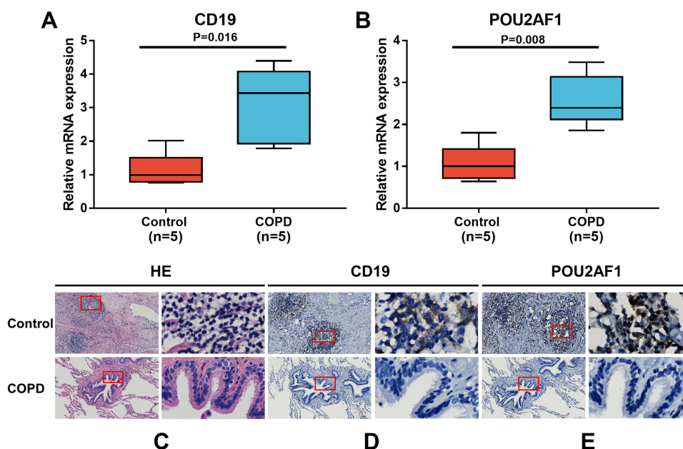
Figure 7 Expression of CD19 and POU2AF1 by qRT-PCR and immunohistochemistry. (A) The mRNA levels of CD19 in human lung tissues. (B) The mRNA levels of POU2AF1 in human lung tissues. The mRNA levels of CD19 and POU2AF1 were normalized to \beta -actin. **P < 0.01 compared with the control group. (C) HE staining in control and patients with COPD. (D) Immunohistochemical staining for CD19 in control and patients with COPD. (E) Immunohistochemical staining for POU2AF1 in control and patients with COPD. Positive protein staining appeared brown and nuclear staining appeared blue. Scale bar = 100 \mu m, original magnification: \times 50 ; scale bar = 10 \mu m, original magnification: \times 400 .
