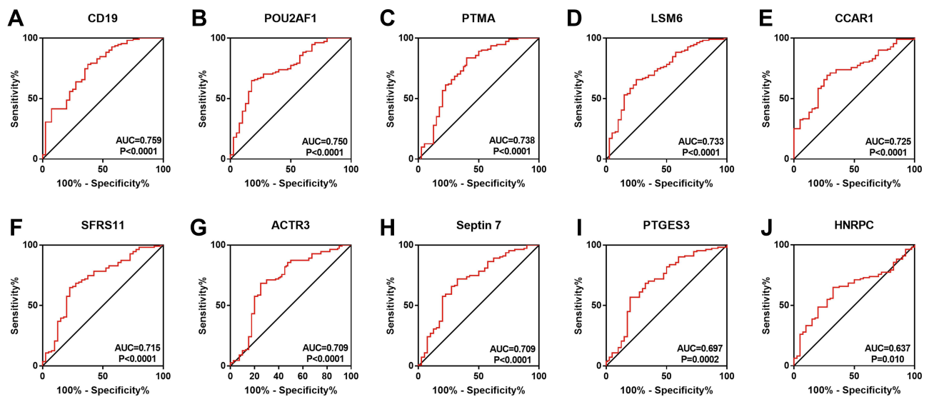
Figure 2 ROC curve of hub genes. The ROC curve of CD19 (A), POU2AF1 (B), PTMA (C), LSM6 (D), CCAR1 (E), SFRS11 (F), ACTR3 (G), Septin7 (H), PTGES3 (I), and HNRPC (J) were represented.
