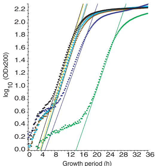
Figure 4. Growth of S.coelicolor J1929 in the presence of different tetracyclines. OD_{492} s of each culture were measured over a period of 50 h. The dots represent the mean growth curves of each condition obtained after synchronization of the replicate cultures to the time point where OD_{492} = 0.04 , as this is the OD when the linear growth begins for nearly all growth curves; the mean OD_{492} at each time point was then calculated, and the values plotted against time. The lines are the averaged regression functions calculated from the linear ranges of each of 48 replicates (two biological replicates). The slope of the mean regression line gave the average growth rate ( \mu_c ), and the extrapolation of the line to where it crossed the x -axis (an OD of 0.005) gave the arbitrary mean lag time ( \lambda_c ). \mu_c and \lambda_c for each condition are shown in Table 3. The mean regression lines and the mean growth curves are colour coded as follows: black, cultures with no addition of inducer; yellow, 0.1 \mu g/ml aTc; light blue, 0.1 \mu g/ml Tc; brown, 1 \mu g/ml aTc; dark blue, 1 \mu g/ml Tc; green, 1 \mu g/ml Dc.
