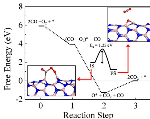
Figure 7. Free energy pathways of CO oxidation on SW-BNNT via LH mechanism. The initial and final states for the desorption of first CO 2 are shown in the lower and upper insets respectively. E a denotes the activation barrier. The sign conventions and atom colors are similar to that followed in Fig. 6. The dotted lines are to guide the eye.
