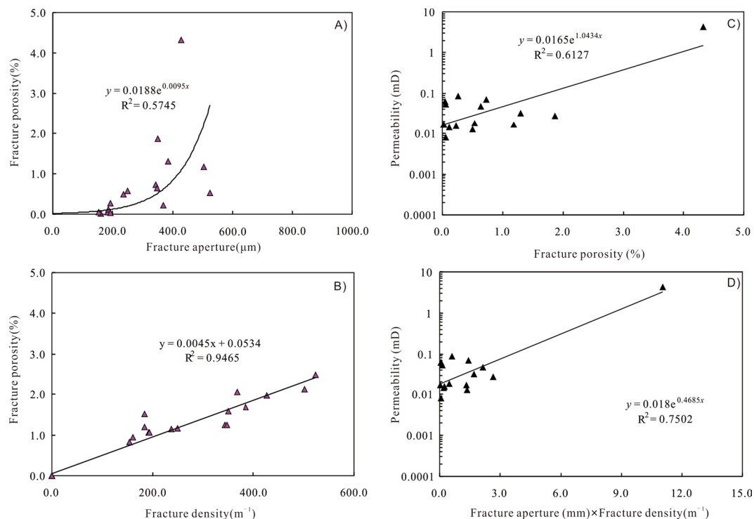
Figure 8. (A) Plot of fracture porosity versus fracture aperture; (B) Plot of fracture porosity fracture density; (C) Plot of horizontal permeability versus fracture porosity; (D) Plot of horizontal permeability versus fracture aperture (mm) multiplied by fracture density ( m^{-1} ).
