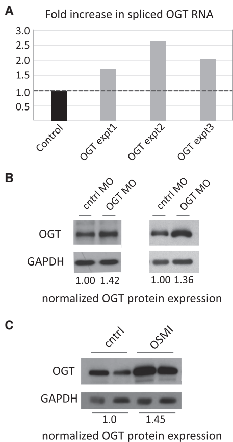
FIGURE 5. Decoy inhibition increases spliced RNA and protein output. (A) Expression of spliced OGT transcript in decoy-inhibited cells, relative to expression in cells treated with a negative control MO. (B) OGT protein expression in two independent experiments was increased in cells treated with the OGT5' decoy MO, compared to cells treated with a control MO. GAPDH expression was used to normalize protein loading. In both experiments inhibition of IR was accompanied by ~1.4-fold increase in protein expression. (C) OGT protein expression in two independent experiments was increased in cells treated with the OGT inhibitor OSMI-1, compared to cells treated with buffer alone.
