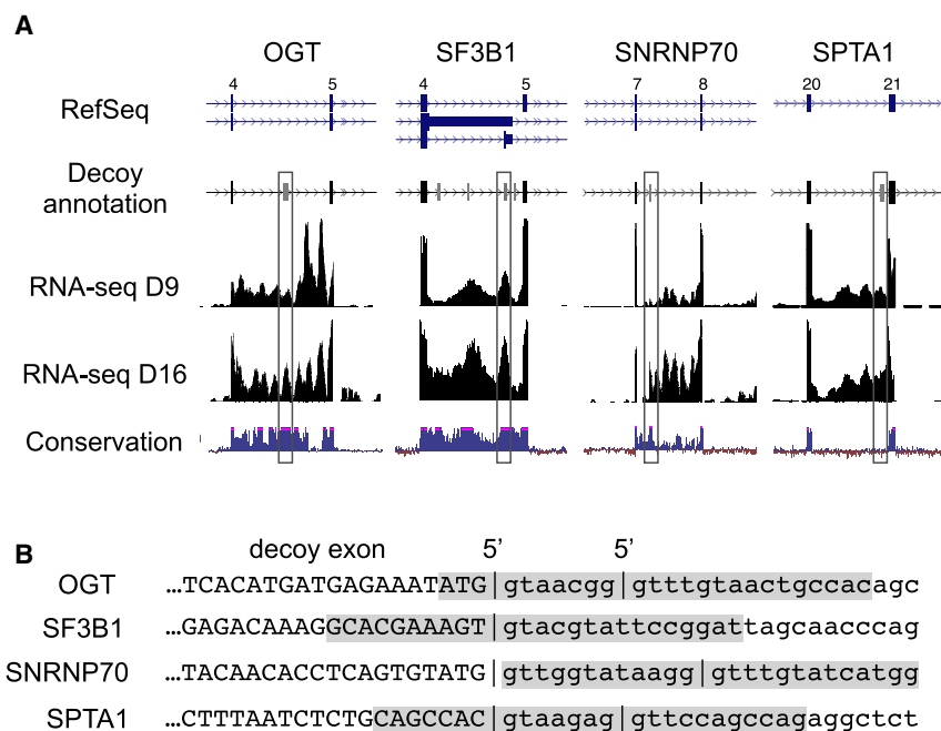
FIGURE 1. Intron retention and candidate decoy exons in targeted erythroid genes. (A) Annotation of key features in IR regions of four prominent erythroid genes. (Top panel) Refseq gene annotations, lacking indications of intron retention isoforms or decoy exons predicted within the introns. For SF3B1, only the four most frequently spliced decoys are shown, from a total of six (Parra et al. 2018). Lower panels show a reannotation that includes predicted decoy exons (boxed), RNA-seq data from early stage (D9) and late stage (D16) erythroblasts, and phylogenetic conservation of the relevant gene regions. (B) 5' splice site features of targeted decoy exons. Upper case, decoy exon sequence; lower case, downstream intron sequence. Vertical bars show 5' splice site junctions identified in RNA-seq data from erythroblasts inhibited for nonsense-mediated decay. Shaded regions indicate regions targeted by antisense MOs.
