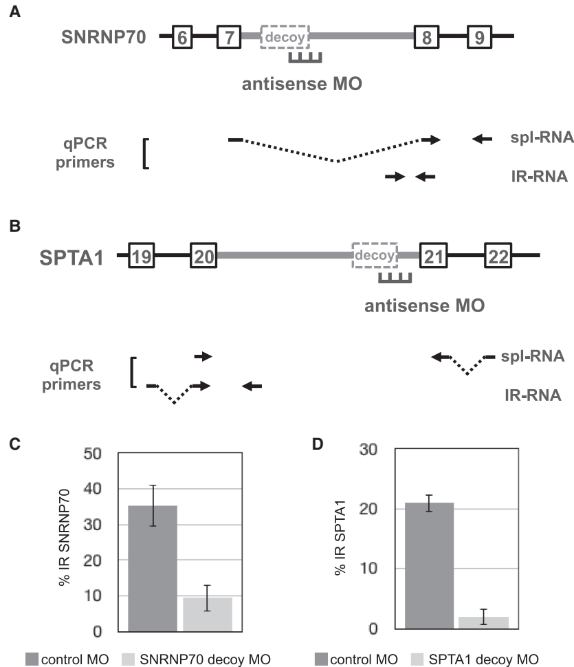
FIGURE 4. Antisense inhibition of SNRNP70 IR and SPTA1 IR. (A) SNRNP70 gene structure in the IR region showing retained intron 7 (thick gray line) with its major decoy exon, together with adjacent introns and exons. Position of antisense MO designed to block the 5' splice site is shown, along with primer pairs used for RT-PCR. (B) SPTA1 gene structure in the IR region showing retained intron 20 (thick gray line) with its major decoy exon, together with adjacent introns and exons. Position of antisense MO designed to block the 5' splice site is shown, along with primer pairs used for RT-PCR. (C,D) IR in cells treated with SNRNP70 -specific (C) or SPTA1 -specific (D) MO, in parallel with cells subjected to control MO treatment. IR was assessed using RT-qPCR to compare the relative amounts of IR and spliced products.
