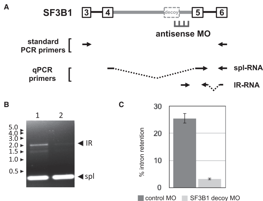
FIGURE 3. Antisense inhibition of SF3B1 IR. (A) SF3B1 gene structure in the IR region showing retained intron 4 (thick gray line) and its major decoy exon, together with adjacent introns and exons. Position of antisense MO designed to block the 5' splice site is shown, along with primer pairs used for RT-PCR. (B) Gel analysis of IR and spliced bands amplified from endogenous SF3B1 transcripts by standard RT-PCR from cells treated with negative control MO (lane 1) or SF3B1 decoy-specific MO (lane 2). (C) SF3B1 IR, as a percentage of total SF3B1 transcripts, in cells treated with negative control or decoy-specific MO. IR was assessed using RT-qPCR to compare the relative amounts of IR and spliced products. Results show average IR of three experiments. Error bars indicate standard deviation.
