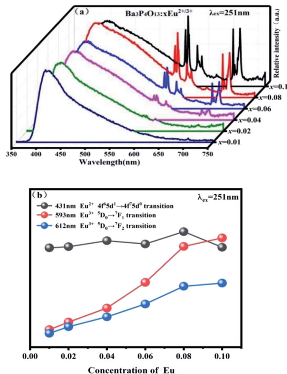
Fig. 7 The emission spectrum of \text{Ba}_3\text{P}_4\text{O}_{13}:\text{xEu} ( x = 0-0.1 ) phosphor under excitation at 251 nm (a) and the emission intensity with peaks at 431 nm, 593 nm and 612 nm as a function of Eu ion concentration (b).
