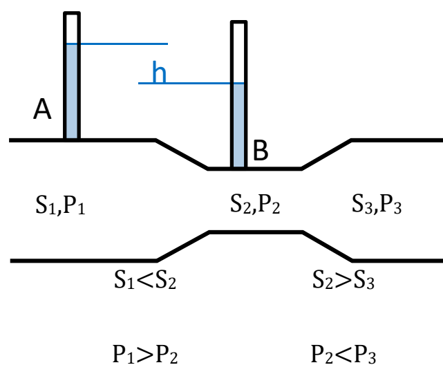
Figure 3. Representation of the Venturi effect. S: speed; P: pressure.
