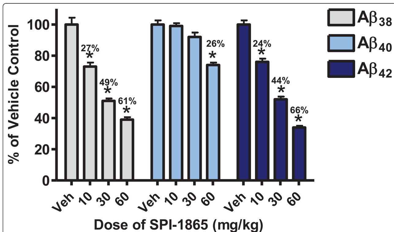
Figure 4 SPI-1865 dose-responsively lowers \beta -amyloid ( A\beta ) _{42} and A\beta_{38} after multiple oral doses. Sprague Dawley rats were orally administered SPI-1865 for six days, once a day (QD) at a dose of 10, 30 or 60 mg/kg. Plasma and brain were harvested 24 hrs post the final dose and analyzed for compound, A\beta_{38} , A\beta_{40} , and A\beta_{42} levels. Data are graphed as a percent of vehicle control. * P -value < 0.01 based on analysis of variance (Dunnett's test).
