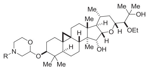
Figure 1 General structure of Satori gamma-secretase modulators (GSMs), including SPI-1865.
