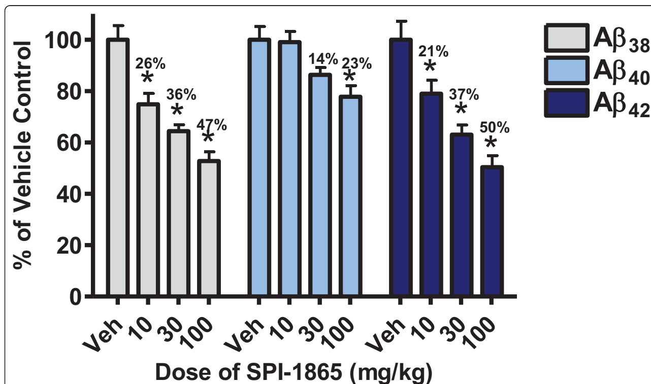
Figure 3 SPI-1865 dose-responsively lowers β-amyloid (Aβ) 42 and Aβ 38 after a single oral dose. Sprague Dawley rats were orally administered a single dose of SPI-1865 of 10, 30 or 100 mg/kg. Plasma and brain were harvested 24 hrs post dose and analyzed for compound, Aβ 38 , Aβ 40 , and Aβ 42 levels. Data are graphed as a percent of vehicle control. *P-value < 0.01 based on analysis of variance (Dunnett's test).
