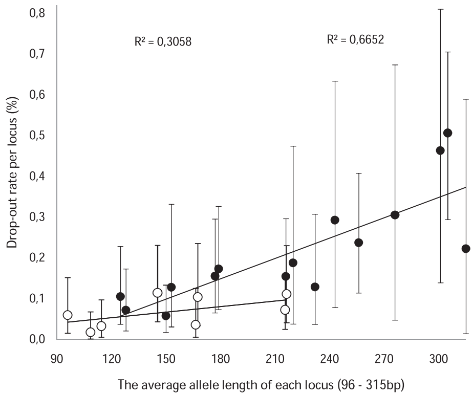
Figure 2 Dropout rates in autosomal short tandem repeat (STR) analyses. IF (black circles) and MF (white circles), plotted against the average allele length of each locus. Limit of detection was 100 relative fluorescence units (RFU).
