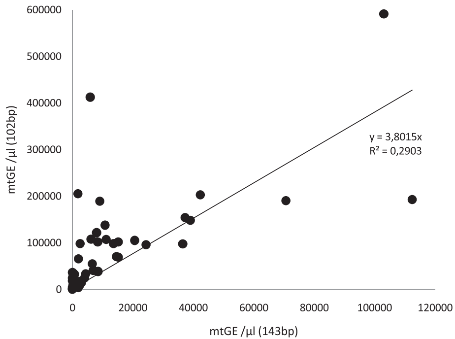
Figure 1 Regression between quantities of mitochondrial genomes (mtGE) measured with amplicons 102 bp and 143 bp in length. The intercept is forced to origin. R^2 is the coefficient of determination of linear regression.
