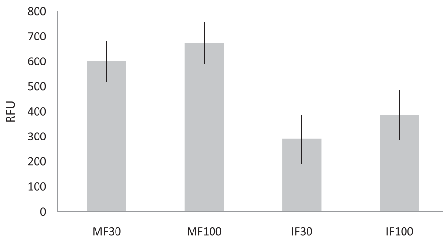
Figure 3 Least squares means of relative fluorescence unit (RFU) values for the nine loci common for both AmpFISTR® Minifiler™(MF) and AmpFISTR® Identifier™(IF) kits. Bars represent 95% confidence intervals in both limits of detection (30 and 100 RFU)
