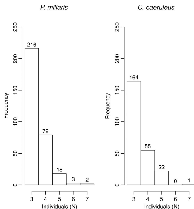
FIGURE 2 The MiMi tool was used to analyse 5,657 potential microsatellite loci discovered in P. miliaris sequence data and 4,513 discovered in C. caeruleus . Loci were filtered to just those which appeared in the sequence data of three or more individuals. The total number of loci which were successfully detected in multiple individuals, and in how many individuals they were detected is shown below. The bar labels are the absolute number of loci that were detected in each category (number of individuals)
