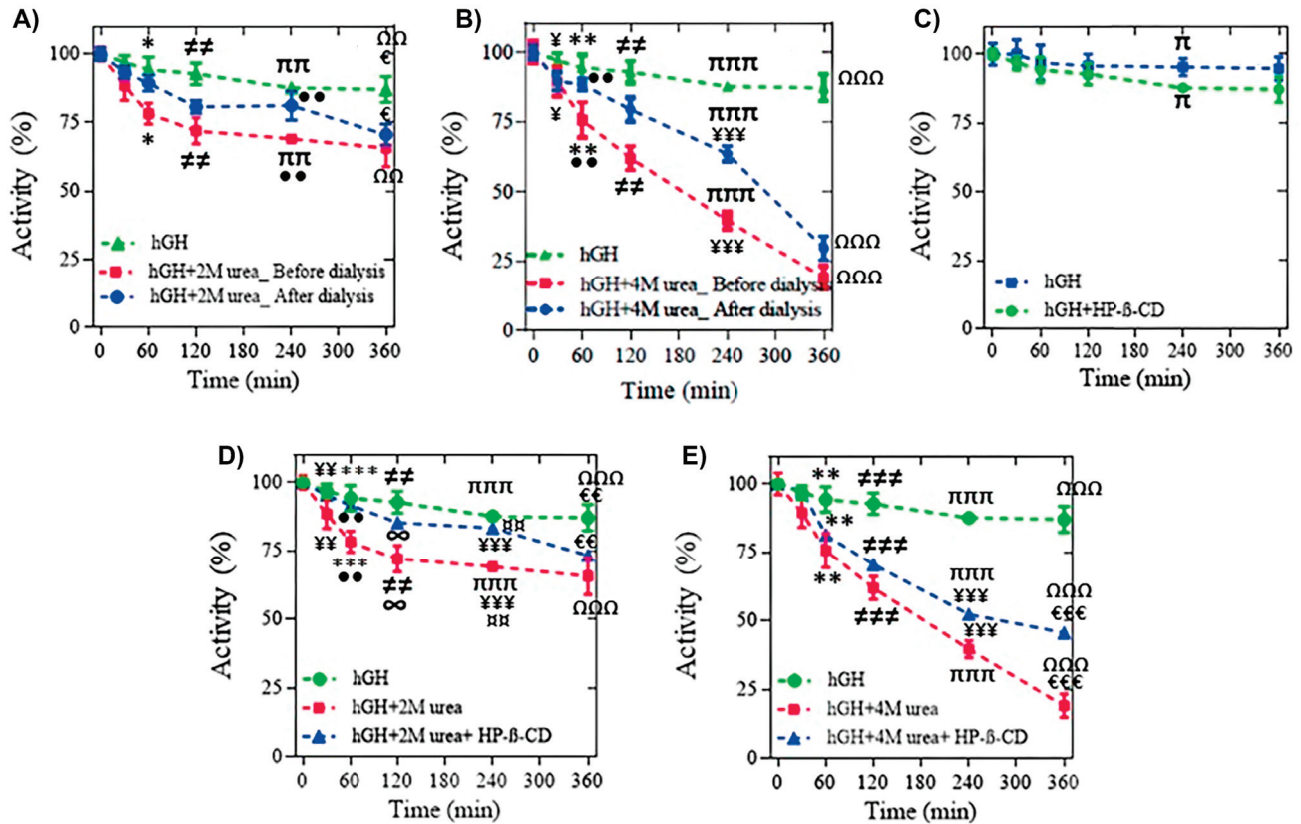
Figure 3. Biological activity of hGH in the presence of A) 2 M urea, B) 4 M urea C) HP- \beta -CD, D) 2 M urea and HP- \beta -CD E) 4 M urea and HP- \beta -CD (Mean \pm SD, N=3, *, \epsilon , \varphi , \pi , \infty P<0.05, \#\# , \pi\pi , \bullet\bullet , \Omega\Omega , \ast\ast , \varphi\varphi , \infty\infty , \epsilon\epsilon P<0.01, \pi\pi\pi , \varphi\varphi\varphi , \Omega\Omega\Omega , \ast\ast\ast , \#\#\# , \varphi\varphi\varphi , \epsilon\epsilon\epsilon P<0.001)
