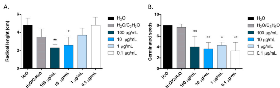
Figure 11. Phytotoxic activity of O. majorana essential oil against radical elongation of L. sativum (A) and against germination of L. sativa (B) seeds. Results are expressed as the mean of three experiments standard deviation. * p < 0.05 , ** p < 0.01 compared to control (ANOVA followed by Dunnett's multiple comparison test).
