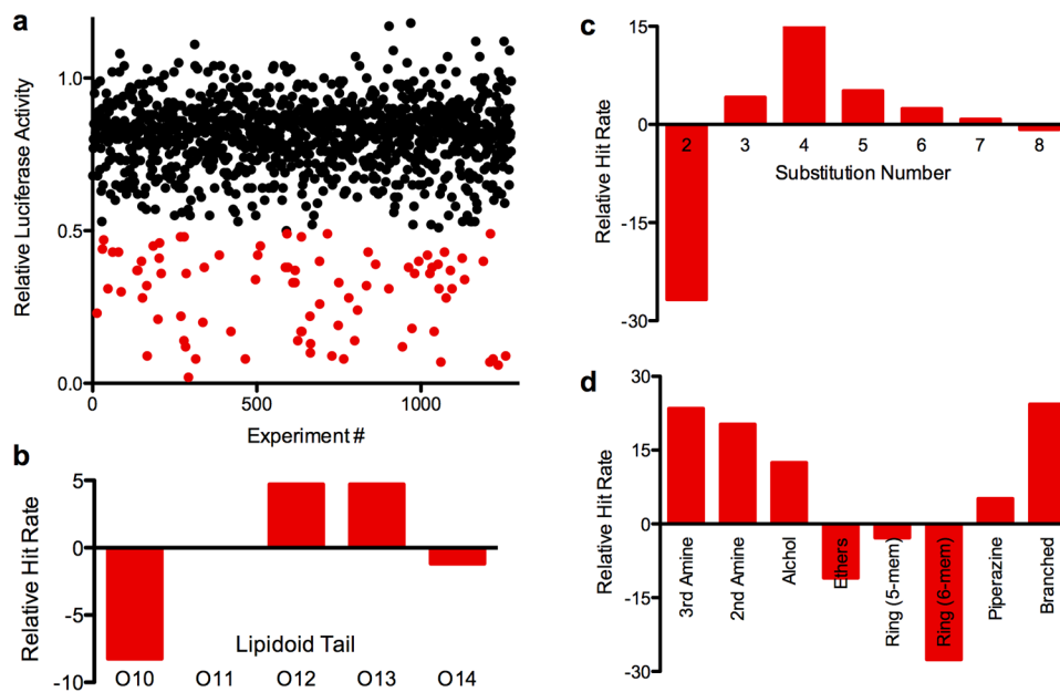
Fig. 2. In vitro siRNA delivery activity of lipidoid nanoparticles
