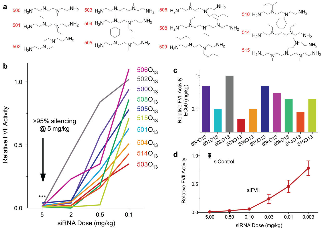
Fig. 5. Lipidoids showed strong structure function relationships in vivo
