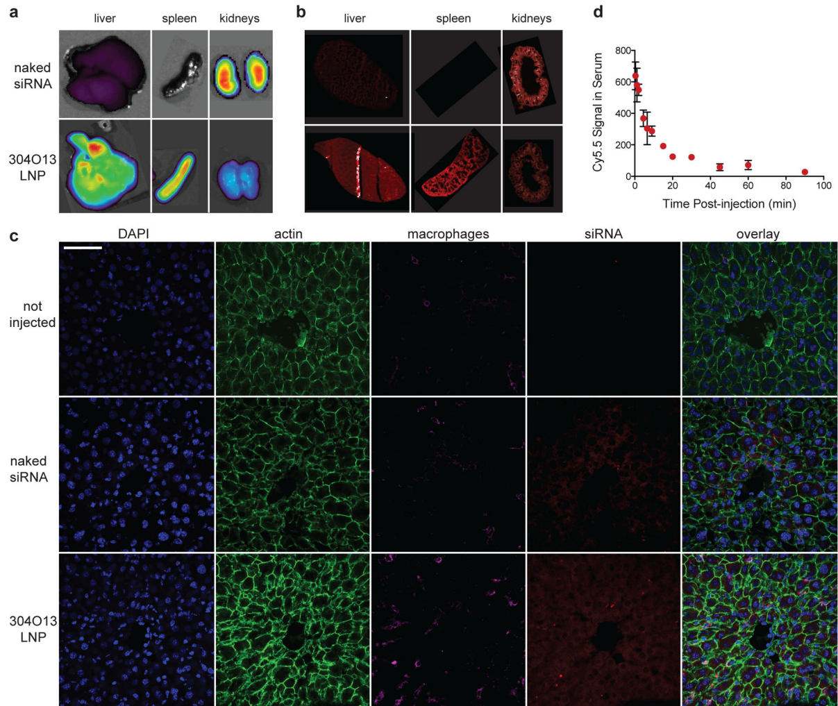
Fig. 4. Biodistribution images for Cy5.5 labeled siRNA delivered with the lipidoid 304O 13 (a) IVIS and (b) Odyssey imaging show that, while naked siRNA is primarily cleared through the kidneys, 304O 13 mediates accumulation in the liver and spleen. (c) Confocal microscopy of 304O 13 – treated liver shows siRNA (red) delivery throughout the tissue, including Kupffer cells (magenta) and hepatocytes (nuclei in blue and actin cytoskeleton in green). Three animals were tested per condition for experiments depicted in panels (a) – (c), and the images shown are representative. Scale bar = 50 μm. (d) 304O 13 LNPs were rapidly eliminated from the bloodstream after tail vein injection. Error bars represent s.d. (n = 3).
