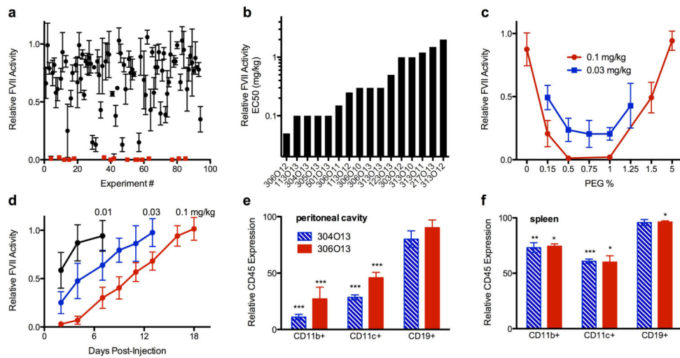
Fig. 3. In vivo siRNA delivery activity of lipidoid nanoparticles
