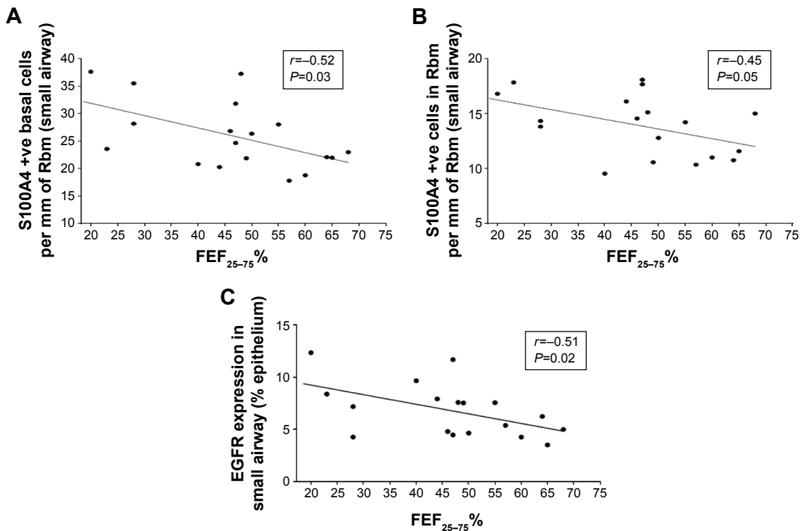
Figure 9 (A) Correlation between the number of small airway basal epithelial cells (per millimeter of Rbm) that were positive for S100A4 with FEF_{25-75}\% (an index of small airway caliber). (B) Correlation between the number of S100A4-positive cells in Rbm (per millimeter of Rbm) in small airway and FEF_{25-75}\% . (C) Correlation between EGFR (% epithelium) in small airway and FEF_{25-75}\% . Abbreviations: EGFR, epidermal growth factor receptor; FEF, forced expiratory flow; Rbm, reticular basement membrane.
