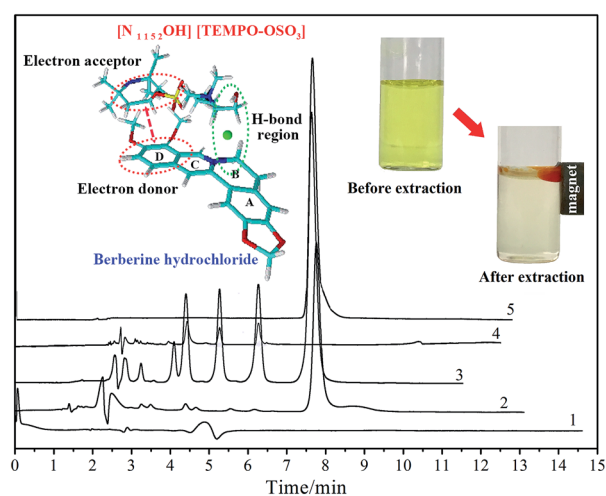
Fig. 4 HPLC chromatograms of [\text{N}_{1.15.2\text{OH}}][\text{TEMPO-OSO}_3] (1), the upper phase (2), crude extract (3), lower phase (4) and berberine hydrochloride standard solution (5), together with molecular simulation results. Mobile phase: 0.1% (V/V) phosphoric acid aqueous solution–methanol (70 : 30); flow rate: 1.0 \text{ mL min}^{-1} ; column temperature: 25^\circ\text{C} ; detection wavelength: 345 \text{ nm} .
